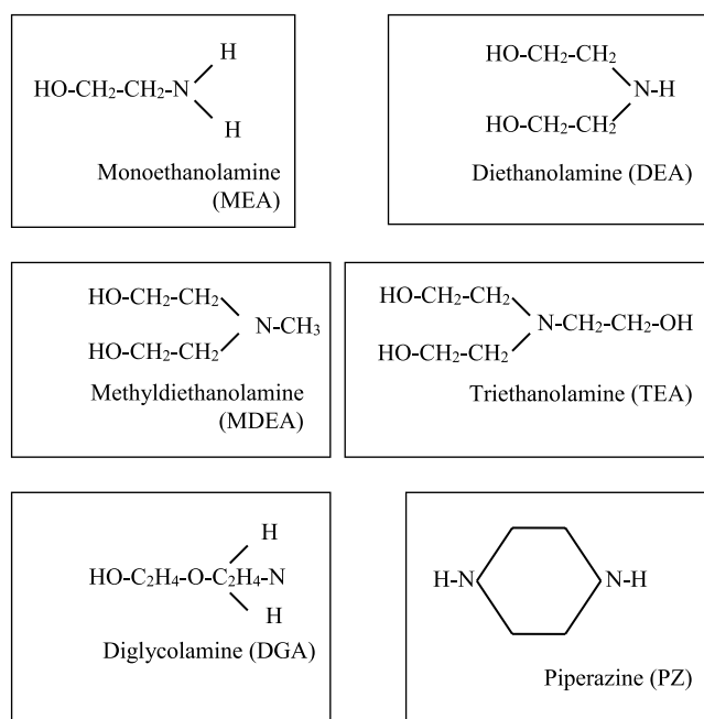
Fig. 1. Chemical structures of most common alkanolamines [1].
