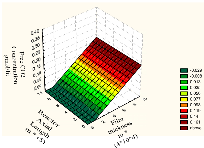
Fig. 13. Surface distribution of free CO 2 concentration in the liquid film for CO 2 fraction 0.1, Q_L = 20 L/hr and CMEA = 3 M as predicted by present model.
