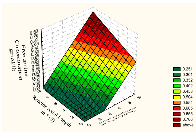
Fig. 15. Linear surface distribution of free amine concentration through the liquid film along the contactor for CO 2 fraction 0.1, Q_L = 20 L/hr and CMEA = 3 M.
