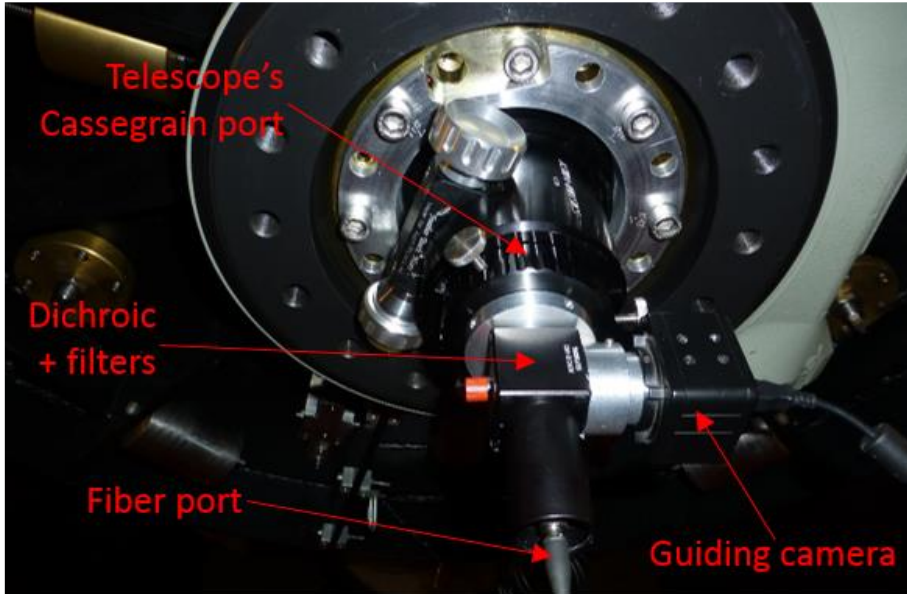
Figure 3: Multi-mode fiber coupling device connected to the C2PU 1-meter telescope’s Cassegrain port through a standard 2-inch eyepiece holder, in which two cascaded focal reducers are placed.
