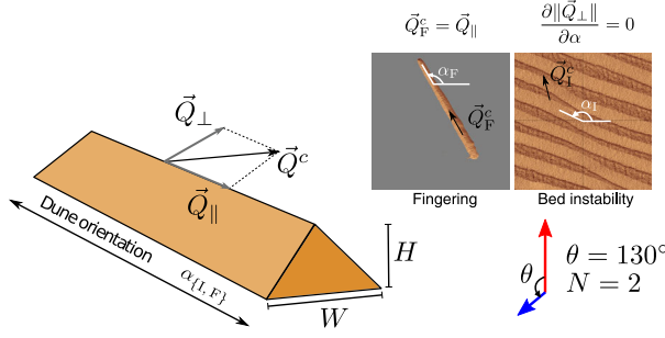
Fig. 18 Dune orientations associated with the bed instability and the fingering modes. The resultant sediment flux \vec{Q}^c at the crest of a dune can be decomposed into two components ( \vec{Q}_{\perp} and \vec{Q}_{\parallel} ) with respect to the dune orientation \alpha . The bed instability orientation corresponds to \partial \parallel \vec{Q}_{\perp} / \partial \alpha = 0 . The fingering mode orientation corresponds to \vec{Q}^c = \vec{Q}_{\parallel} and \parallel \vec{Q}_{\perp} \parallel = 0 . Numerical examples are shown for a divergence angle \theta = 130^\circ and a transport ratio N = 2 between the two winds Gao et al. (2015). The dominant and secondary winds are shown using red and blue arrows, respectively. Note that, given the speed-up effect in multi-directional wind regimes, the resultant sand flux at the crest of dunes in the bed instability and fingering modes ( \vec{Q}_I^c and \vec{Q}_F^c ) may differ not only in intensity but also in orientation (du Courrech et al. 2014)
