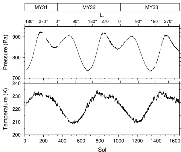
Fig. 2 Pressure and temperature recorded by the REMS instrument suite on board the Mars Science Laboratory (Curiosity Rover). Sol is relative to the landing date. Pressure and temperature data were averaged on a per-sol basis, where sols with incomplete data coverage being removed from the plot. The temperature and pressure seasonal cycles are clearly evident
