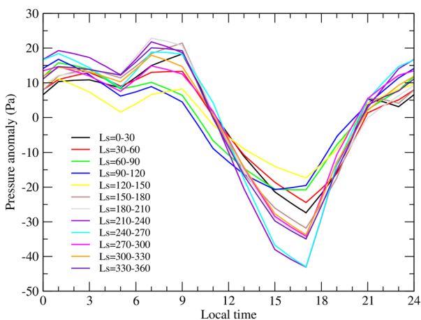
Fig. 7 The diurnal oscillation of surface pressure (difference with diurnal mean value) at the Insight landing site as predicted by the LMD Global Climate Model (twelve values per day are included). This shows the signature of the diurnal and semi-diurnal thermal tide
