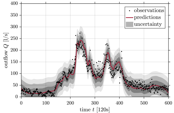
Figure 11: Corrected predictions.
