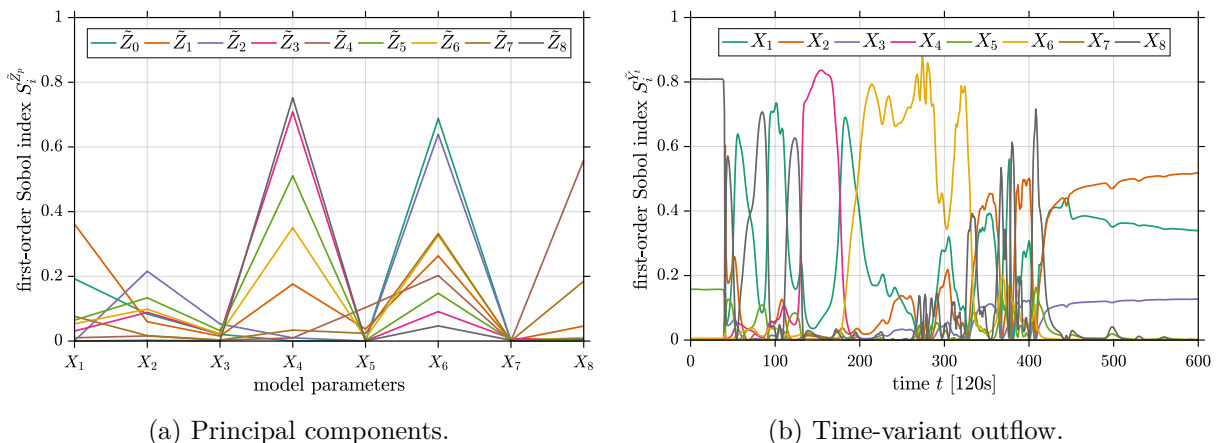
Figure 6: First-order Sobol indices.
