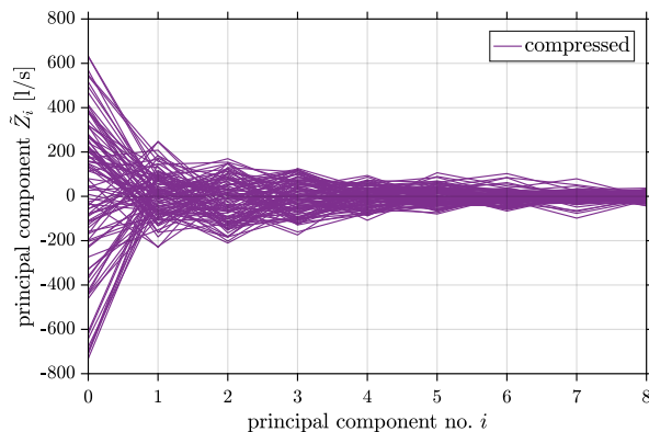
Figure 3: Principal component analysis.
