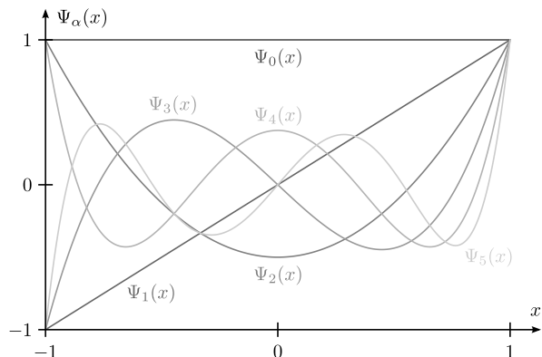
Figure 4: Legendre polynomials.
