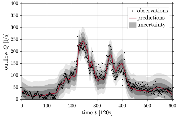
Figure 11: Corrected predictions.
