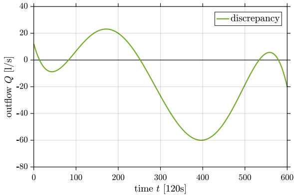
Figure 10: Model discrepancy.
