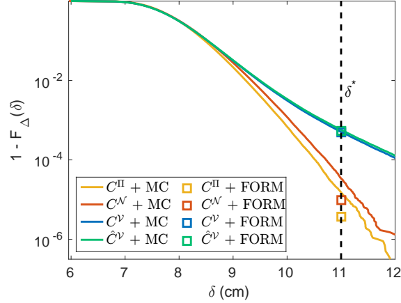
Figure 4: Reliability analysis of the truss structure. Solid lines: MC estimate of the survival function \mathbb{P}(\Delta > \delta) for loads coupled by the independence copula C^{(\text{II})} (yellow), the Gaussian copula C^{(\text{N})} (red), the C-vine with known parameters C^{(\text{V})} (blue, mostly overlapping with green), and the C-vine with fitted parameters \hat{C}^{(\text{V})} (green). The vertical dashed line marks the critical threshold \delta^* . Squares: estimates of P_f obtained by FORM.
