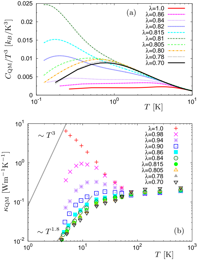
FIG. 17. Temperature dependence of (a) C_{\text{QM}}/T^3 and (b) \kappa_{\text{QM}} at the indicated values of \lambda . The specific heat C_{\text{QM}} (Eq. (27)) is calculated from the g(\omega) data of Fig. 6. The thermal conductivity \kappa_{\text{QM}} is obtained by applying Eq. (28) to the MD data of Fig. 15(b). For those calculations, we have used physical Argon units, \sigma = 3.405 \text{ \AA} , \epsilon/k_B = 125.2 \text{ K} , and \tau = 2.11 \text{ ps} . In the figures, the temperature, specific heat, and thermal conductivity are measured in units of K, k_B , and \text{Wm}^{-1}\text{K}^{-1} , respectively. For \lambda \leq 0.86 , \kappa_{\text{QM}} increases as \kappa_{\text{real}} \propto T^\gamma with \gamma = 1.8 \simeq 2 , and a plateau value is observed around T \sim 20 \text{ K} . The excess peak in C_{\text{QM}}/T^3 , however, is found in the lower temperature region T \leq 1 \text{ K} . A discussion of this point is included in the text.
