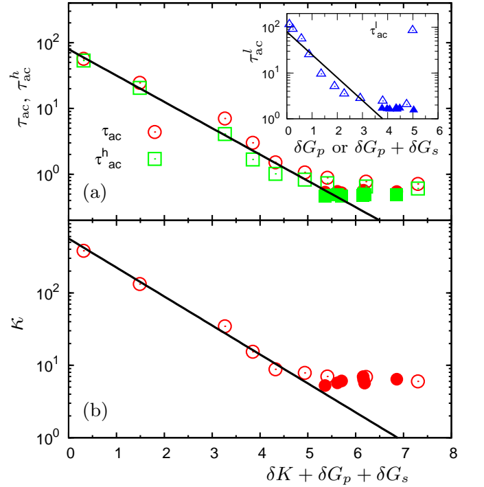
FIG. 14. (a) The life-times \tau_{\text{ac}}, \tau_{\text{ac}}^h, \tau_{\text{ac}}^l of the acoustic waves, averaged over the entire, high ( \omega > 5 ) and low ( \omega < 5 ) frequency ranges, respectively, as detailed in the text. In the main panel, the data of \tau_{\text{ac}} and \tau_{\text{ac}}^h are plotted as functions of the extent of the elastic heterogeneities, \delta K + \delta G_p + \delta G_s , for \lambda \geq \lambda^* (open symbols) and \lambda < \lambda^* (closed symbols). The line is an exponential fit \tau_{\text{ac}} \simeq \tau_{\text{ac}}^h \sim \exp[-(\delta K + \delta G_p + \delta G_s)/g_\tau] , with g_\tau \simeq 0.4 . In the inset, we plot \tau_{\text{ac}}^l as a function of \delta G = \delta G_p + \delta G_s for \lambda \geq \lambda^* (open symbols) and \delta G = \delta G_p + \delta G_s for \lambda < \lambda^* (closed symbols). The solid line is a fit of the form \tau_{\text{ac}}^l \sim \exp[-\delta G/g_{\tau^l}] with g_{\tau^l} \simeq 0.5 . (b) The thermal conductivity \kappa shown as a function of the extent of the elastic heterogeneity, together with an exponential fit \kappa \sim \exp[-(\delta K + \delta G_p + \delta G_s)/g_\kappa] , with g_\kappa \simeq g_\tau \simeq 0.4 . Note that in the highly disordered states with large values of \delta K + \delta G_p + \delta G_s , both \tau_{\text{ac}} and \kappa reach the minimum allowed values, where the life-time \tau_{\text{ac}} \sim \mathcal{O}(10^{-1}) is the Einstein period 102,103 , and the mean-free-path of the acoustic waves is of the order of the particles diameter.
