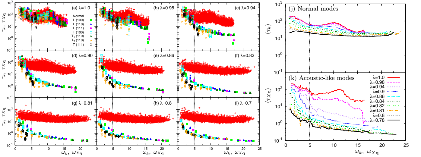
FIG. 12. Left panel: Life-times of the normal modes \tau_k , and of the acoustic-like waves \tau_{Xq} , plotted as functions of \omega_k and \omega_{Xq} , respectively, at the indicated values of \lambda . Here we consider the longitudinal ( L ) and transverse ( T ) acoustic waves propagating in the (100), (110), and (111) directions (see Fig. 11). Specifications of the different data sets are shown in the key. The vertical lines indicate \omega = 5 for reference. In the perfect crystalline state \lambda = 1 , \tau_k \simeq \tau_{Xq} , while in defective and disordered states, life-times of acoustic-like modes strongly deviate from those pertaining to normal modes. For \lambda \leq 0.86 , the \tau_{Xq} at high frequencies are of the order of the minimum time scale set by the Einstein period \tau_E . This is the typical time scale of the thermal motion of particles, and was estimated as \tau_E \simeq 10^{-1} for the present soft-sphere system 102,103 . Right panel: The averaged life-times of the normal vibrational modes \langle \tau_k \rangle (j), and of acoustic plane waves \langle \tau_{Xq} \rangle (k), versus the frequency \omega_k and \omega_{Xq} , respectively, at the indicated values of \lambda . These data are the same as those shown in the left panels, averaged in bins of width \Delta\omega = 1 , and over all considered propagation directions and polarizations. A comprehensive discussion of these data is included in the main text.
