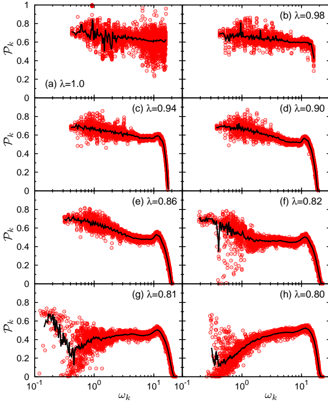
FIG. 7. Participation ratios, \mathcal{P}_k , versus the eigenfrequencies, \omega_k , at the indicated values of \lambda . The solid lines represent the averaged values \langle \mathcal{P}_k \rangle calculated by smoothing the data in bins of width \Delta\omega = 0.015 . A detailed discussion of these data is given in the main text.
