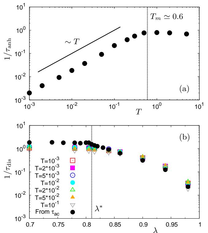
FIG. 16. (a) T -dependence of the anharmonic term, 1/\tau_{anh} (Eq.(23)) at \lambda = 1 , and (b) \lambda -dependence of the disorder term, 1/\tau_{dis} (Eq.(24)) at the indicated values of T . The vertical line indicates the melting temperature T_m \simeq 0.6 at \lambda = 1 in (a), and the transition point \lambda^* in (b). In (b) we also plot (closed black circles) the values extracted from the life-times \tau_{ac} shown in Fig. 14(a) by using Eq.(25). We can see that 1/\tau_{dis} does not depend on temperature for T \leq 10^{-1} , and there is a good agreement with the values extracted from \tau_{ac} . This observation supports the validity of the additive decomposition of the attenuation of Eq. (22).
