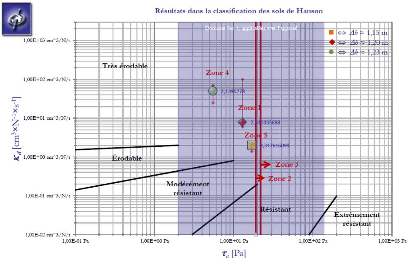
Figure 5. Erosion parameters provided from Geophyconsult company, from the tests performed on the experimental dike sections. Zones 4 and 5 are related to untreated soil, Zones 2 and 3 to lime-treated soil. Vertical red lines are estimates of the lowest critical stress values, as no significant erosion was observed on these lime-treated zones.
