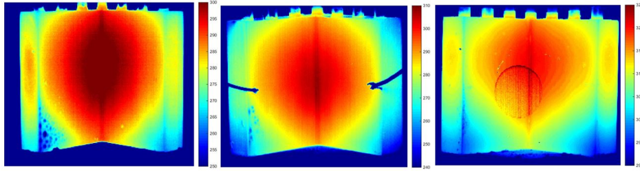
Figure 2: Infrared thermography in front of the internal surfaces of the T-square black painted at 300°C for the three spectral ranges: 0.9 \mu\text{m} to 1.7 \mu\text{m} (left picture), 3 \mu\text{m} to 5 \mu\text{m} (central picture) and 8 \mu\text{m} to 12 \mu\text{m} (right picture)
