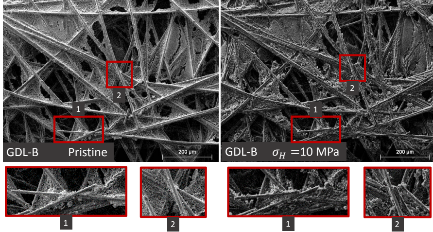
Figure 6: SEM images of the GDL-B, in a pristine state (left) and after applying a compression pressure of 10 MPa (right). Magnified images on two locations are shown on the bottom of the figure where fibers breakage are occurring.
