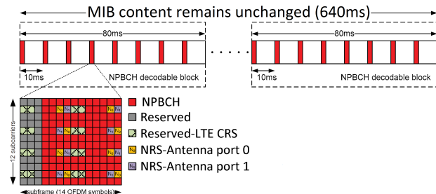
Fig. 18. NPBCH Transmission [45]
