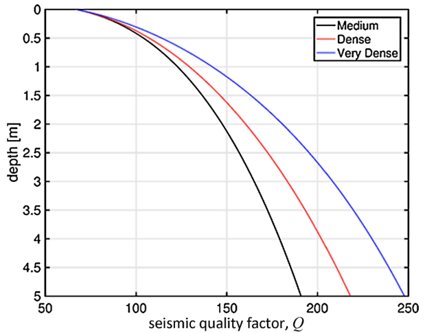
Fig. 12 Models of Q as a function of depth for the upper five meters of regolith at the InSight landing site. The three profiles correspond to the density profiles shown in Fig. 3 based on different states of regolith compaction
