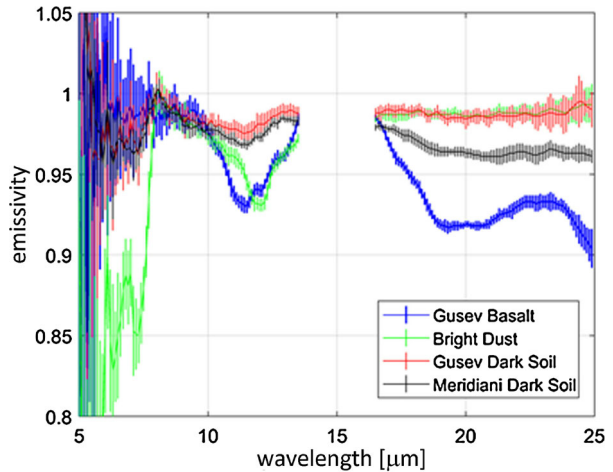
Fig. 6 Emissivity spectra from the Spirit and Opportunity Mini TES instrument (Ruff et al. 2006). Blue: Gusev basalt (2t 131344843 emr 1151 p3175 n0 a1). Green: bright dust (2t 133288501 emr 2232 p3654 n0 a1). Red: Gusev dark soil (2t 130533990 emr 09 br p3156 n0 a1). Black: Meridiani Planum dark soil (1t 132362778 emr 05 am p3217 n0 a1)
