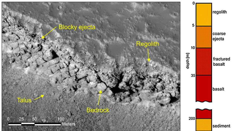
Fig. 2 Left: An example of the shallow structure of the InSight landing site. HiRISE image PSP_002359_2020 of a portion of the exposed steep scarp of the Hephaestus Fossae in southern Utopia Planitia at 21.9°N, 122.0°E showing \sim 10 m thick, fine grained regolith, that grades into coarse, blocky ejecta that overlies strong, jointed bedrock (arrows show each). Right: Stratigraphic model of the shallow subsurface in the InSight landing region based on geological interpretation of orbital data and analysis of rocky crater ejecta. Figure modified from Knapmeyer-Endrun et al. (2017)
