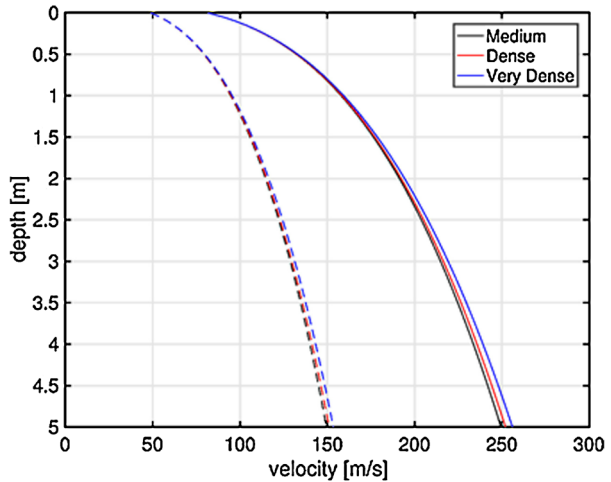
Fig. 10 Model P- and S-wave velocities as a function of depth for the upper five meters of regolith at the InSight landing site. The three profiles correspond to the density profiles shown Fig. 3 based on different states of regolith compaction. Solid lines indicate v_P and dashed lines v_S
