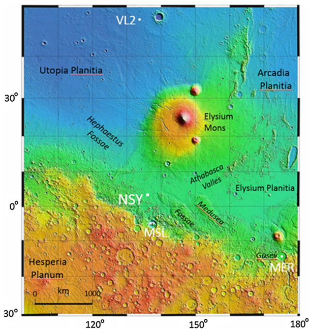
Fig. 1 Topographic map of the region around the InSight landing site (NSY) showing major physiographic features, mentioned in the text, as well as the Viking Lander 2 (VL2), Mars Science Laboratory (MSL), and Mars Exploration Rover (MER) Spirit landing sites. Spirit landed in Gusev crater and Curiosity (MSL) landed in Gale crater. The map is a portion of the Mars Orbiter Laser Altimeter (MOLA) topographic map of Mars (Smith et al. 2001)
