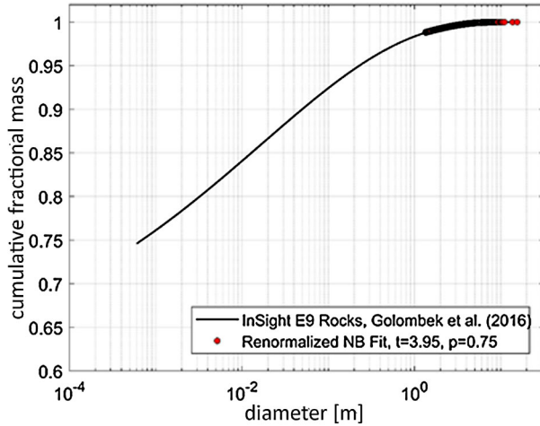
Fig. 5 Plot of the cumulative fractional mass versus diameter of the rocks measured above the resolution limit at the InSight landing ellipse E9. The rocks are shown in red, while the negative binomial (NB) fit and prediction to the rock data distribution and below is shown in black. The mass estimation assumes spherical particles and constant density and it is renormalized to match the observable cumulative fractional area (CFA), as previously reported by (Golombek et al. 2017). The NB fit is extrapolated down to 600 \mu\text{m} —a reported upper size limit for saltation (Kok et al. 2012)—and estimates an approximate value of mass at 75% below this limit
