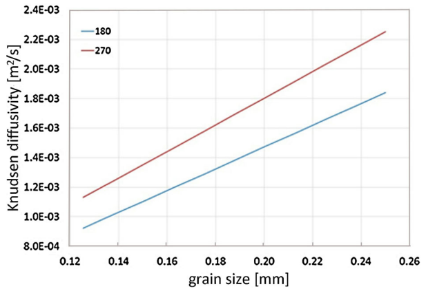
Fig. 14 Knudsen Diffusivity (Pressure diffusion coefficient) versus regolith grain size for regolith and atmospheric conditions likely to occur at the InSight landing site. The numbers given by the key to the curves are temperature in Kelvin
