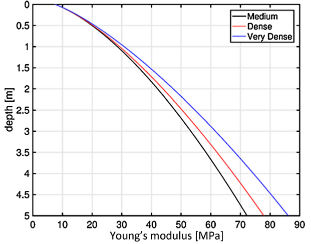
Fig. 11 Models of Young’s modulus as a function of depth for the upper five meters of regolith at the InSight landing site. The three profiles correspond to the density profiles shown in Fig. 3 based on different states of regolith compaction
