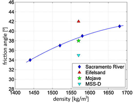
Fig. 4 Change in friction angle with density of the Sacramento River sand (Lee and Seed 1967) compared to friction angles obtained with a direct shear box on various Mars regolith simulants by Delage et al. (2017). The Sacramento River sand has rounded particles that are closer in shape to Martian regolith than the simulants considered here. A friction angle around 28–30° is estimated at the surface of the InSight landing place. The changes in density with depth shown in Fig. 3 provide a negligible increase at 5 m in the medium case, and an increase up to 36° in the very dense case
