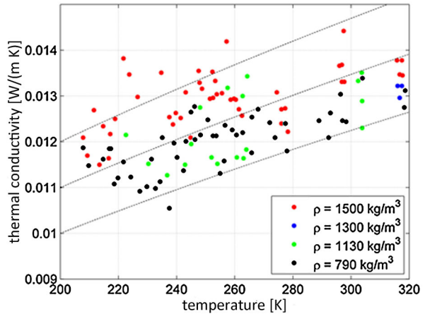
Fig. 8 Comparison between thermal conductivity measurements of 37–62 \mu\text{m} particles of basalt under 7 hPa of \text{CO}_2 gas as a function of the temperature by Fountain and West (1970) (dots) and thermal conductivity trend modeled using (6) (dashed lines)
