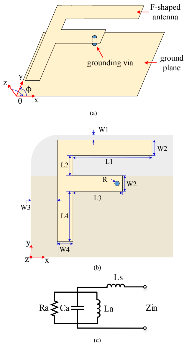
Figure 2. Geometries and an equivalent circuit of the proposed F-shaped antenna: (a) 3-D view with substrate board removed; (b) Top view; (c) The equivalent circuit of the antenna.
