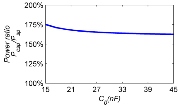
Fig. 10. Power improvement of CSP-OSECE versus V_{oc,org} in comparison with SP-OSECE.
