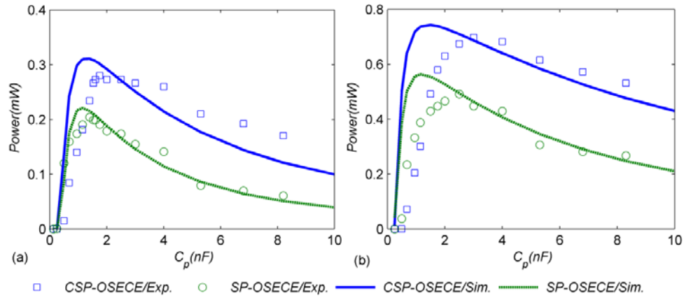
Fig. 5. Power results of both circuits with various C_p and constant R_{load} : (a) a single piezoelectric patch ( C_0=14\text{nF} ); (b) two piezoelectric patches ( C_0=28\text{nF} ).
