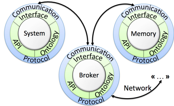
Fig. 1. The MBA architecture proposed in this research.
