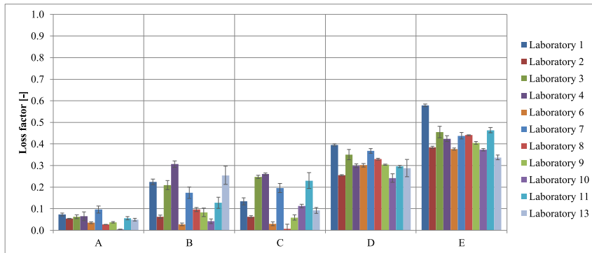
Fig. 13. Comparison in terms of mean value and standard deviation of η for all laboratories and materials.
