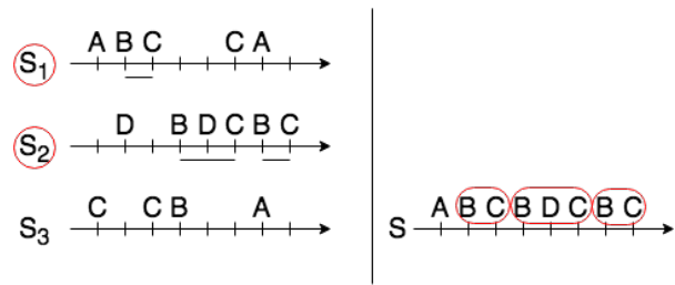
Figure 2: Occurrences of BC as sequential pattern (left) and episodes (right). The occurrences are coloured in red. The sequential pattern BC has 2 occurrences in the left dataset, while the episode BC has 3 occurrences in the right dataset.
