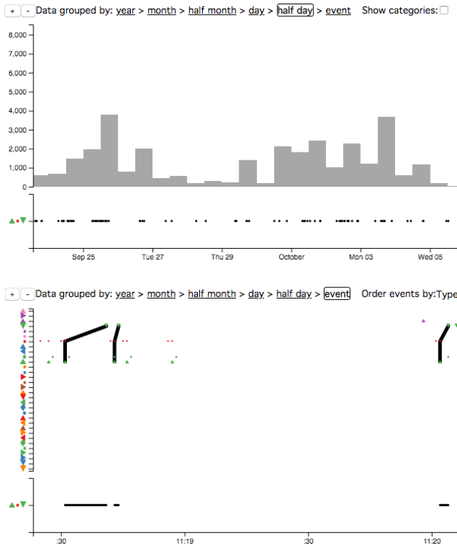
Figure 6: Visualizations of a pattern's occurrences. Depending on the zoom level, the analyst can either see an overview of where the occurrences are (black dots on the top image) or a detailed view of the events composing the occurrences (linked events on the bottom image).
