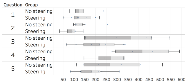
Figure 8: Summary of time needed for participants to perform the tasks. Graduations are in seconds.
