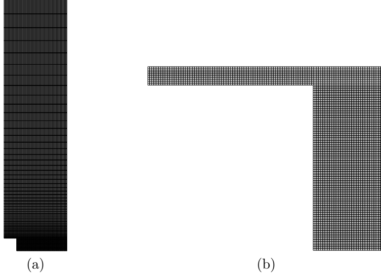
Fig. 3. Two examples of meshes used in the finite element calculations. Eight-node quadratic elements. (a) Mesh of the unit cell in the case W = 1 , \chi = 0.2 and c = 0.05 . (b) Mesh of the unit cell in the case W = 1 , \chi = 0.7 and c = 0.9 .
