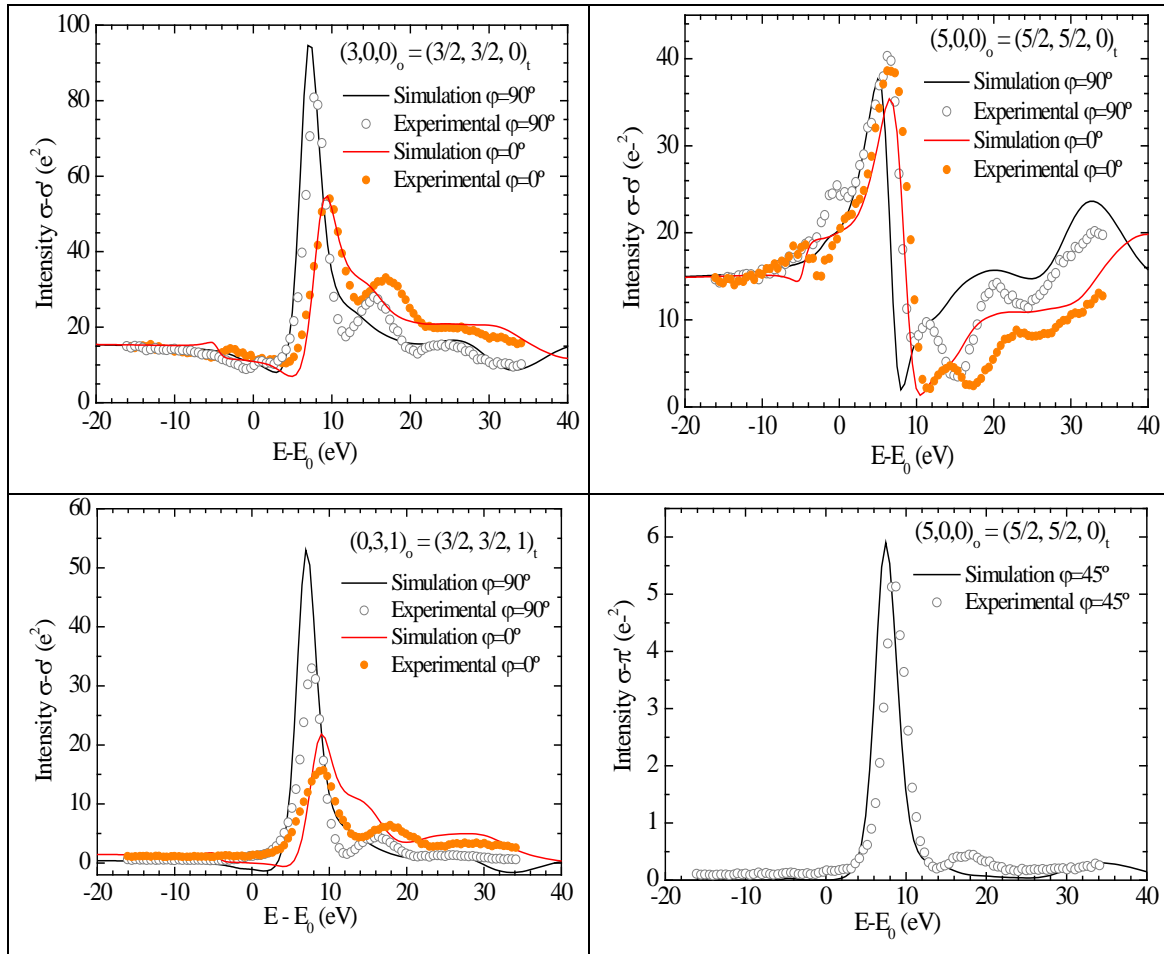
Figure 9. Energy dependence of theoretical simulated intensities (full line) and self-absorption corrected experimental RXS spectra (dots) for the resonant reflections in \text{La}_{1.5}\text{Ca}_{0.5}\text{CoO}_{4.02} around the Co K-edge. Theoretical simulations are performed with the oxygen atom displacements relative to the A2mm structure of \text{Cd}_2\text{CoO}_4 given in the text.
