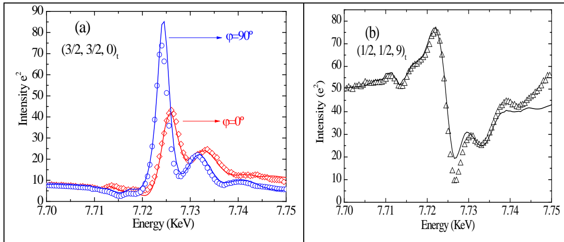
Figure 7. Comparison between the self-absorption corrected energy dependence of resonant reflections (points) and the simulated spectra (lines) obtained from the empirical analysis outlined in the text in the \sigma - \sigma' channel for (a) the (3/2, 3/2, 0)_t reflection of the \text{La}_{1.6}\text{Ca}_{0.4}\text{CoO}_{4.04} sample at \varphi=90^\circ ( \mathbf{E} // \mathbf{c} ) and \varphi=0^\circ ( \mathbf{E} \perp \mathbf{c} ) and (b) the (1/2, 1/2, 9)_t of the \text{La}_{1.3}\text{Ca}_{0.7}\text{CoO}_{3.9} sample at \varphi=90^\circ .
