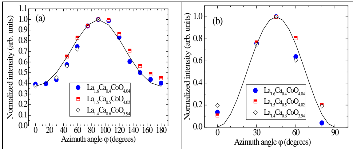
Figure 4. Normalized azimuthal dependence of the resonant intensity at E=7.7245 keV for (a) the (3/2, 3/2, 0)_t reflection in the \sigma - \sigma' channel and (b) the (5/2, 5/2, 0)_t reflection in the \sigma - \pi' channel for \text{La}_{2-x}\text{Ca}_x\text{CoO}_{4\pm\delta} ( x=0.4, 0.5 and 0.6 ). The data were normalized to the values at \phi=90^\circ and at \phi=45^\circ for the \sigma - \sigma' and \sigma - \pi' resonant intensities, respectively. The solid lines are the results of calculations by Eq. [1] and [2], as discussed in the text.
