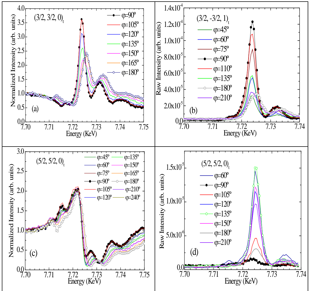
Figure 1. Energy-dependence of resonant reflections near the Co K-edge as a function of the azimuth angle without absorption correction: (a) (3/2, 3/2, 0)_t ; (b) (3/2, -3/2, 1)_t and (c) (5/2, 5/2, 0)_t in the \sigma - \sigma' polarization channel and (d) (5/2, 5/2, 0)_t in the \sigma - \pi' polarization channel for the \text{La}_{1.5}\text{Ca}_{0.5}\text{CoO}_{4.02} single crystal.
