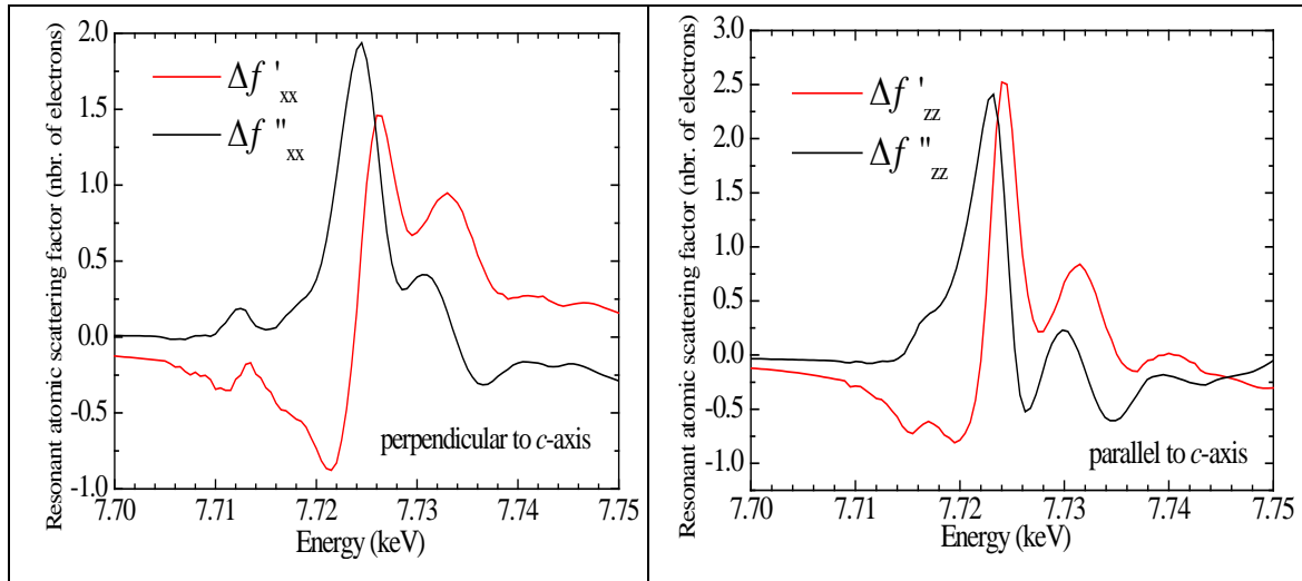
Figure 5. (a) The real ( \Delta f'_{xx} ) and imaginary ( \Delta f''_{xx} ) terms of the difference of the resonant atomic scattering factors for Co1 and Co2 atoms when the polarized electric field \mathbf{E} is perpendicular to the c -axis. (b) The real ( \Delta f'_{zz} ) and imaginary ( \Delta f''_{zz} ) components of the difference of the resonant atomic scattering factors for Co1 and Co2 atoms when the polarized electric field \mathbf{E} is parallel to c -axis.
