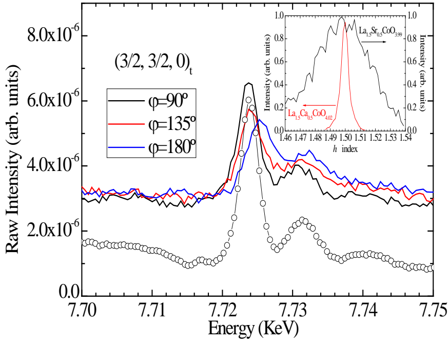
Figure 3. Energy dependence of the raw intensity at the (3/2, 3/2, 0)_t reflection in the \sigma - \sigma' channel without absorption correction for \text{La}_{1.5}\text{Sr}_{0.5}\text{CoO}_{3.99} (solid lines). The energy dependence of the raw intensity at the same reflection and \varphi=90^\circ in the \sigma - \sigma' channel without absorption correction for \text{La}_{1.5}\text{Ca}_{0.5}\text{CoO}_{4.02} divided by a factor 50 is also shown for comparison (open circles). Inset. h -scans through the (h, h, 0)_t CO reflections for the \text{La}_{1.5}\text{Ca}_{0.5}\text{CoO}_{4.02} and \text{La}_{1.5}\text{Sr}_{0.5}\text{CoO}_{3.99} samples normalized at the peak position. Correlation lengths were extracted from the scans by a Lorentzian fit to be \xi(\text{La}_{1.5}\text{Ca}_{0.5}\text{CoO}_{4.02}) \sim 219 \text{ \AA} and \xi(\text{La}_{1.5}\text{Sr}_{0.5}\text{CoO}_{3.99}) \sim 21 \text{ \AA} .
