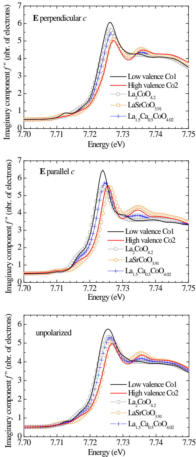
Figure 8. Imaginary f''(E) components of the resonant atomic scattering factor of the two Co sites with the electric field parallel to the ab -plane (upper panel), the electric field parallel to the c -axis (middle panel) and unpolarized (bottom panel) compared to the corresponding experimental XANES spectra of the \text{La}_2\text{CoO}_{4.2} , \text{La}_{1.5}\text{Ca}_{0.5}\text{CoO}_{4.02} and \text{LaSrCoO}_{3.91} samples normalized to electron units.
