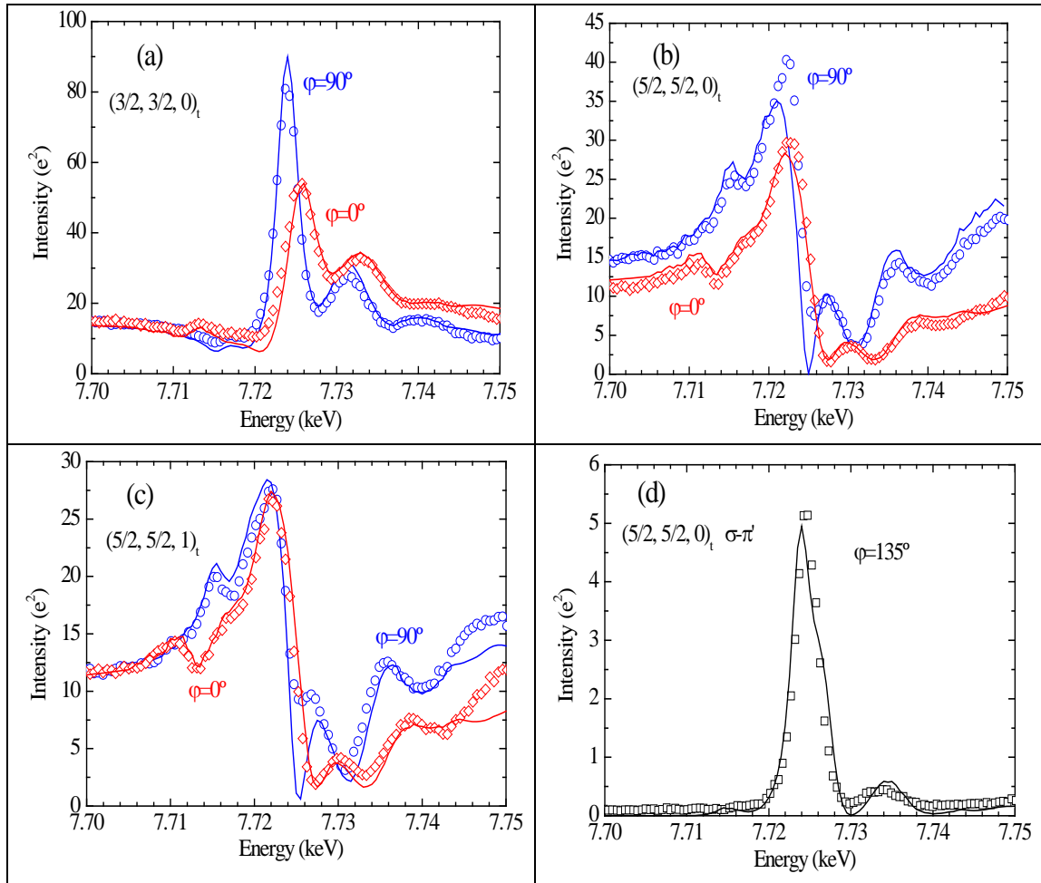
Figure 6. Comparison between the self-absorption corrected energy dependence of resonant reflections (points) and the simulated spectra (lines) obtained from the empirical analysis outlined in the text for the \text{La}_{1.5}\text{Ca}_{0.5}\text{CoO}_{4.02} sample. (a) Data for (3/2, 3/2, 0)_t reflection in the \sigma\text{-}\sigma' channel at \varphi=90^\circ ( \mathbf{E}//\mathbf{c} ) and \varphi=0^\circ ( \mathbf{E}\perp\mathbf{c} ). (b) Data for (5/2, 5/2, 0)_t and (c) for (5/2, 5/2, 1)_t reflections in the same polarization channel and azimuth angles. (d) Data for (5/2, 5/2, 0)_t reflection in the \sigma\text{-}\pi' channel at \varphi=135^\circ .
