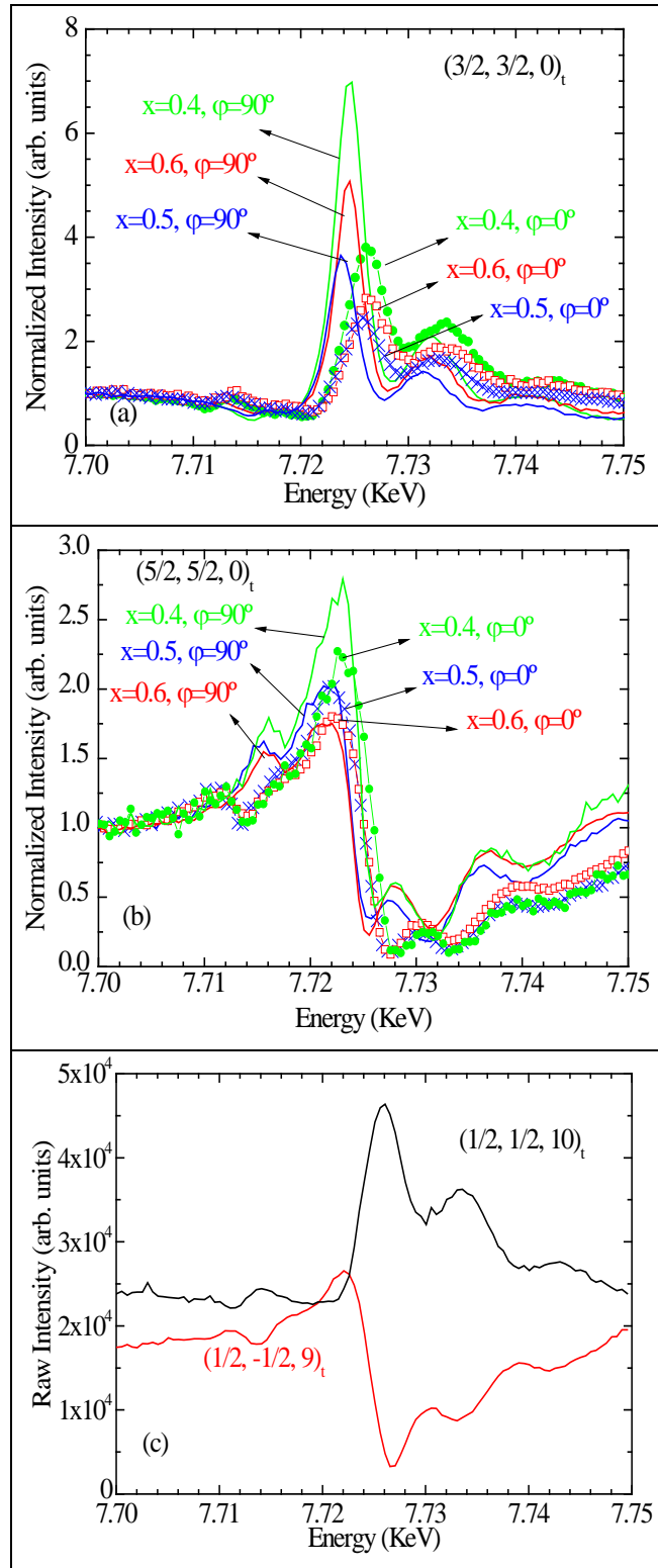
Figure 2. Energy dependence of the resonant (3/2, 3/2, 0)_t (a) and (5/2, 5/2, 0)_t (b) reflections for \text{La}_{2-x}\text{Ca}_x\text{CoO}_{4\pm\delta} ( x=0.4, 0.5, 0.6 ) samples at two azimuth angles with \mathbf{E} \parallel \mathbf{c} ( \varphi=90^\circ ) and \mathbf{E} \perp \mathbf{c} ( \varphi=0^\circ ) in the \sigma - \sigma' channel without absorption correction. c) Energy dependence of the resonant (1/2, -1/2, 9)_t and (1/2, 1/2, 10)_t reflections for the \text{La}_{1.3}\text{Ca}_{0.7}\text{CoO}_{3.9} sample at \varphi=90^\circ in the \sigma - \sigma' channel without absorption correction.
