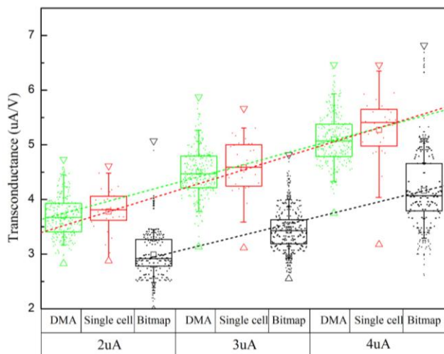
Fig. 11. Transconductance measured at 2, 3 and 4 uA for single cells (on 36 device), DMA on test chip (256 bits), and bitmap (2048 bits) using equivalent reading conditions.
