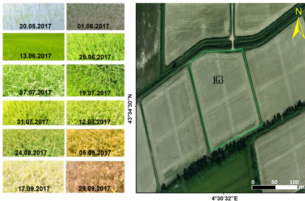
Figure 3. The reference plot 1G3 is marked in the figure (coordinates of central point 43^{\circ}34'30''N , 4^{\circ}30'32''E ) together with its photos at different dates.
