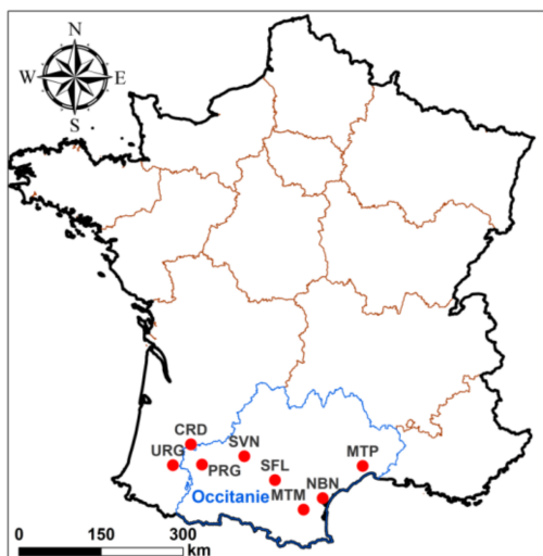
Figure 1. Location of the 7 stations of SMOSMANIA network (Narbonne “NBN”, Mouthoumet “MTM”, Saint-Félix-Lauragais “SFL”, Savenès “SVN”, Peyrusse “PRG”, Creon d’Armagnac “CRD”, Urgons “URG”), and the center of the site located near Montpellier city (MTP, 12 km × 12 km) where additional measurements were obtained. In situ measurements of MTP and NBN were not considered if the corresponding pixel of a SSM product covers the sea water.
