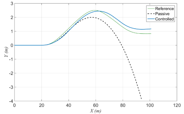
Figure 26. Vehicle trajectories.
