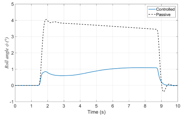
Figure 31. Roll angle \phi .
