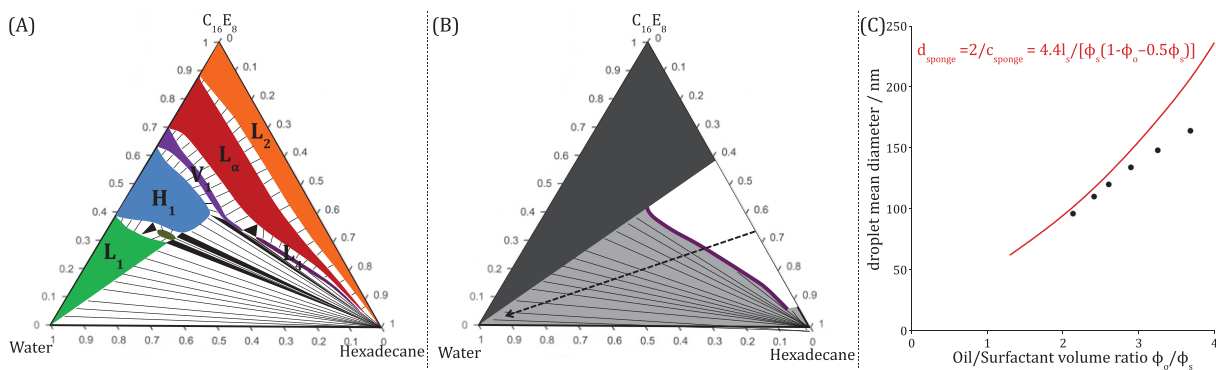
Fig. 3. (A) Phase diagram at T = 50^\circ\text{C} of the C_{16}E_8 /water/hexadecane ternary system. L_2 : reverse droplet-like microemulsion, L_\alpha : lamellar phase, L_4 : direct bicontinuous sponge phase, V_1 : bicontinuous cubic phase, H_1 : hexagonal phase, L_1 : direct droplet-like microemulsion. (B) Simplified diagram showing in white the initial compositions that lead to a successful nanoemulsification upon rapid water addition and in gray the unsuccessful ones. The line separating the two domains is the locus of the sponge phase L_4 . (C) Variation of the droplet mean diameter with the oil/surfactant ratio in the case of a successful emulsification. This requires a starting composition in the white area of (B) and thus a pathway that crosses the sponge phase. The red line is the calculation from the curvature of the surfactant film in this sponge phase. It matches quantitatively the experimental data with no fitting parameters and thus demonstrates that the sponge phase templates the final nanoemulsion. Source: Data from Roger et al. [25].
