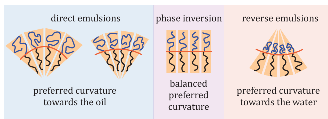
Fig. 1. The preferred curvature of the surfactant layer can be turned towards the oil, yielding direct self-assembly structures and emulsions, or turned towards the water, yielding reverse self-assembly structures and emulsions. Phase inversion occurs when the preferred curvature is zero. The preferred curvature can be tuned for example by changing the interactions between the hydrophilic head and water or adding water to a water deprived surfactant layer.
