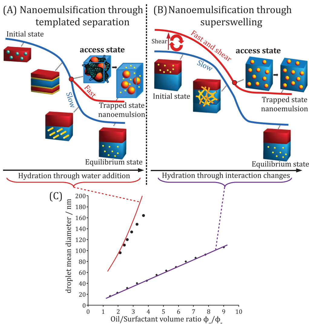
Fig. 4. Summary of the two mechanisms of nanoemulsification through the disruption of bicontinuous structures. Data from Roger et al. [24,25]. (A) Water is added to a homogeneous bicontinuous network the curvature of which is already turned towards the oil. Oil phase separates within this network and the droplets adopt the sponge phase's curvature before being trapped in a metastable state by further dilution. Some surfactant is wasted as small micelles in water. (B) The interactions between the surfactant head and water are modified so that the preferred curvature matches the geometrical curvature. Shearing the system in this location of the parameter space breaks the equilibrium bicontinuous network coexisting with excess oil and water into a dispersion of oil-superswollen micelles, named superswollen microemulsion. All the surfactant is used at the interfaces. (C) Mean droplet diameter for nanoemulsions produced through the two mechanisms. For nanoemulsification through templated phase separation, the diameter is given by the curvature of the sponge phase. Droplets are much smaller for nanoemulsification through superswelling since all the surfactant is efficiently used. The diameter is then given by the geometrical curvature.
