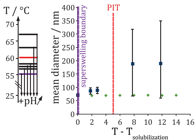
Fig. 5. Original data. Mean diameter of nanoemulsion droplets prepared either by a rapid pH increase in a mixed surfactant system C_{16}E_8 /oleic acid (blue squares) or a rapid cooling for a pure surfactant system C_{16}E_8 (green diamonds), from various initial states controlled by the temperature. For the pure system, all the initial states located at or above the superswelling boundary give the same nanoemulsion, the droplets of which are at the geometrical curvature. For the mixed system, this ideal nanoemulsion is only obtained if the starting point is on the superswelling boundary where the access state is formed. If the temperature is increased a few degrees above a coarser emulsion is obtained. If the temperature is increased above the phase inversion, a very coarse emulsion is obtained. Phase inversion is then not only useless but damaging to the success of the process.
