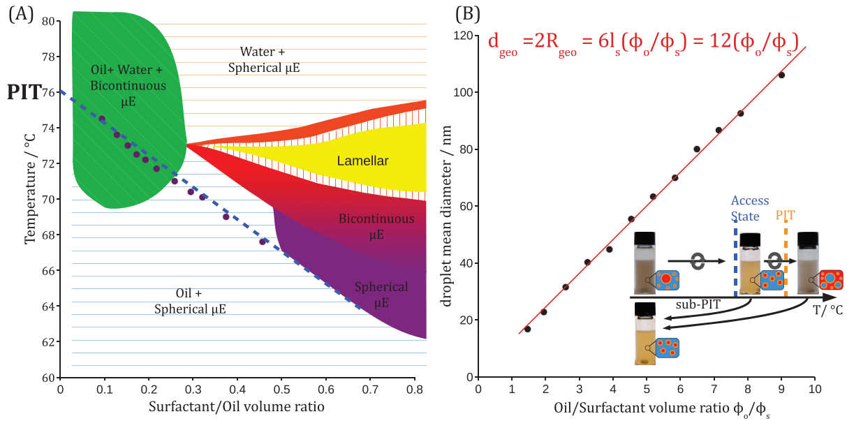
Fig. 2. (A) Cut of the equilibrium phase prism at constant oil/water ratio. The purple dots correspond to the superswelling boundary at which all the oil is solubilized into micelles under shear. The blue line corresponds to the equality between the geometrical curvature and the preferred curvature and matches this experimental superswelling boundary. (B) Mean droplet diameter as a function of the oil/surfactant ratio corresponding to rapid cooling from the purple dots on the superswelling boundary. The orange line represents the calculation of the geometrical radius and also matches the experimental data with no fitting parameter. The insert displays the visual aspect of the sample through the temperature cycle and the corresponding microstructure. Cooling from the superswelling boundary or from above the phase inversion temperature yielded the same nanoemulsion for this pure ternary system C_{16}E_8 /water/hexadecane. Source: Data from Roger et al. [24].
