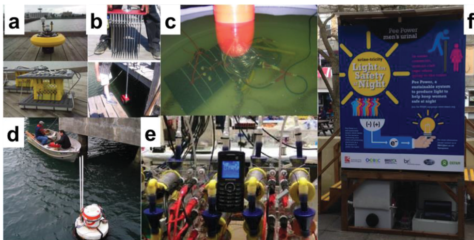
Fig. 8. Images of the benthic microbial fuel cell done by Prof. Tender group (a,b) and by Prof. Beyenal group (c,d). A basic mobile phone charged by a stack of 12 ceramic microbial fuel cells (e), and the Pee Power™ urinal tested on the University of the West of England, Bristol campus (f). (Fig. 8a, b adapted from Ref. [461] with permission of Elsevier, Fig. 8c, d Photo Credit: Prof. Zbigniew Lewandowski and Prof. Haluk Beyenal, Fig. 8e Adapted from Ref. [473], published by the PCCP Owner Societies, CC BY 3.0 ( https://creativecommons.org/licenses/by/3.0/ )).
