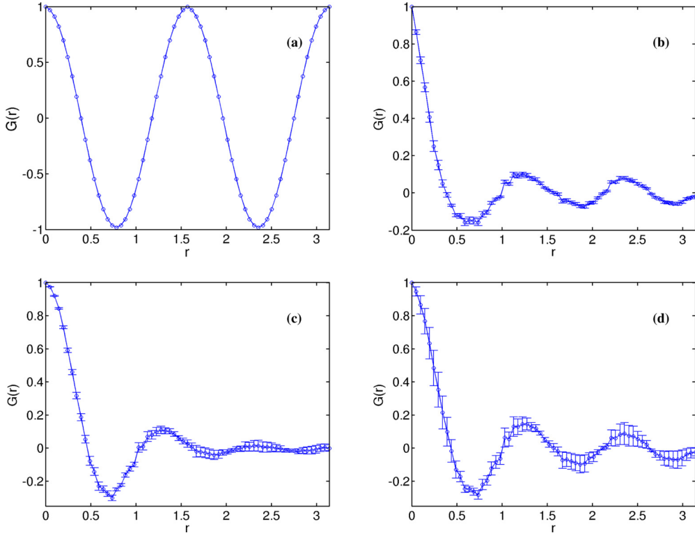
FIG. 13. (a) Plot of G(r) for the crystalline state with \Omega = 1 and Wi = 1 along the line connecting \mathbf{r} = (\pi/2, \pi/2) and \mathbf{r} = (\pi/2, \pi) ; and plots of the circularly averaged G(r) in the turbulent state with (b) \Omega = 1 and Wi = 20 , (c) \Omega = 22 and Wi = 0 , and (d) \Omega = 22 and Wi = 20 .
