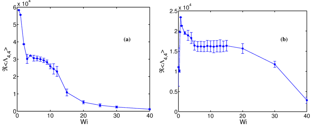
FIG. 12. Plots of \langle \hat{\Lambda}_{k=(4,4)} \rangle versus Wi for (a) \Omega = 1 and for (b) \Omega = 22 ; in (b) \langle \hat{\Lambda}_{4,4} \rangle first increases with Wi , goes through a maxima, which corresponds to an OPXA state, and then decreases after that.
