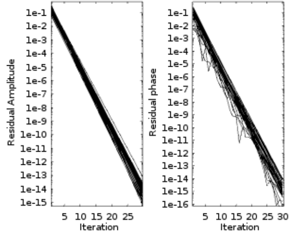
Fig. 8. Amplitude and phase of the difference between the estimated gains at iteration x and the true gain vector in a 40 antenna scalar calibration case
