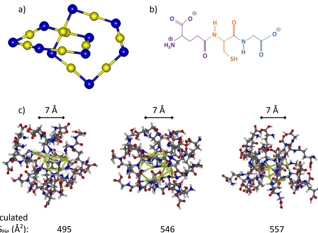
Figure 1: (a) schematic model of catenane structures : [5,5] (interconnected rings of Au 5 S 5 ). (b) chemical structure of the glutathione tripeptide ligand : \gamma -L-Glutamyl-L-cysteinylglycine. (c) PM7 optimized catenane-like structures for Au 10-12 SG 10-12 . Grey lines are drawn on the core structure of Au 10 SG 10 to highlight the catenane structure. CCS values calculated, from the neutral form of catenane-like structures with the trajectory method, are also given.
