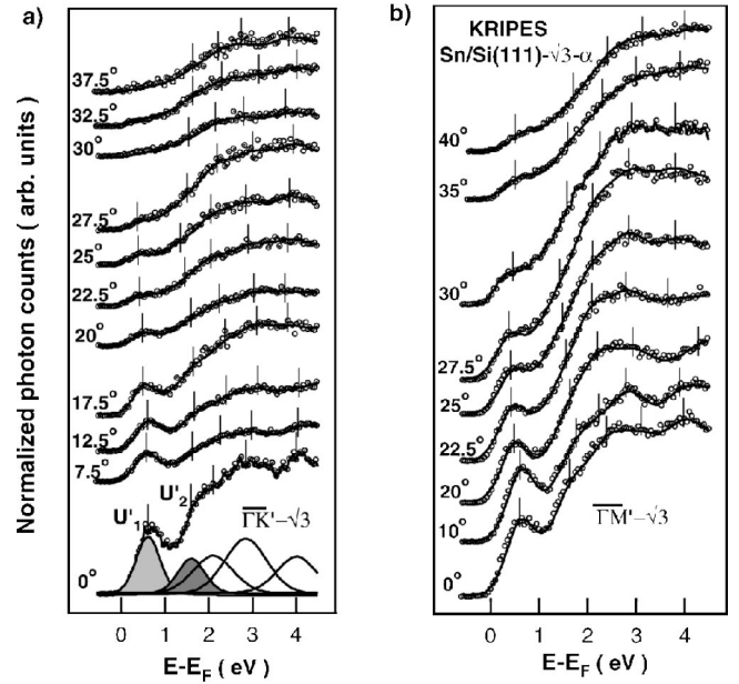
FIG. 3. KRPES spectra of the \alpha - \sqrt{3} surface along the \overline{\Gamma K'} (a) and \overline{\Gamma M'} (b) directions of the SBZ for selected angles of the incident electrons. Experimental curves are plotted as circles, the fit is represented by a continuous line, and each Gaussian maximum is marked by a vertical bar.
