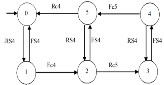
c4: Detector of the turntable loading position c5: Detector of the turntable unloading position S4: Turntable
