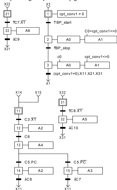
Fig. 7. Functional specification (GRAFCET) of the sorting system
