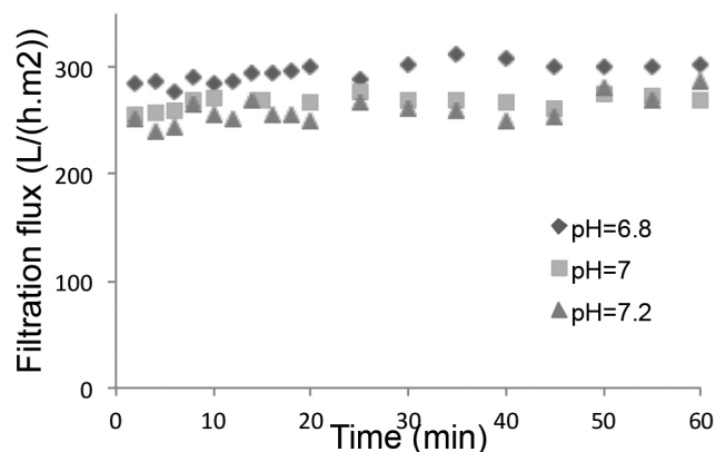
Fig. 5. Influence of the pH on the variation of the filtration flux with time, hybrid process, [\text{Fe}^{2+}]_0 = 10 \text{ mg}\cdot\text{L}^{-1} , \text{TMP} = 0.6 \text{ bar} .
