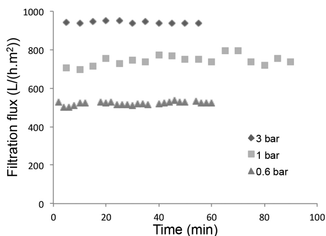
Fig. 7. Influence of TMP on the variation of filtration flux with time, hybrid process, [\text{Fe}^{2+}]_0 = 10 \text{ mg}\cdot\text{L}^{-1} , \text{pH} = 7 .
