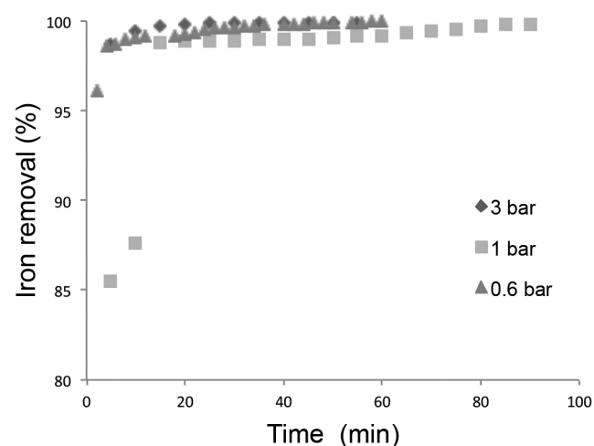
Fig. 6. Influence of TMP on the variation of iron removal with time, hybrid process, [\text{Fe}^{2+}]_0 = 10 \text{ mg}\cdot\text{L}^{-1} , \text{pH}=7 .
