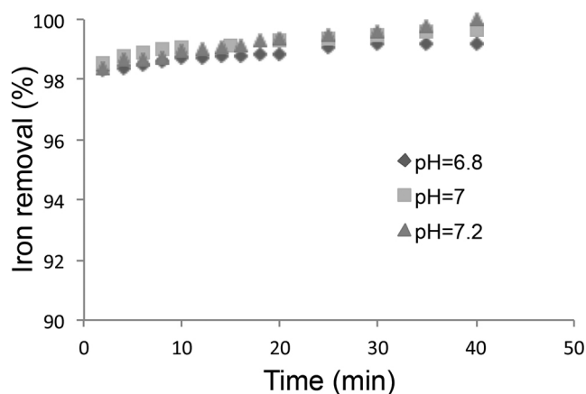
Fig. 4. Influence of the pH on the variation of iron removal with time, hybrid process, [\text{Fe}^{2+}]_0 = 10 \text{ mg}\cdot\text{L}^{-1} , \text{TMP} = 0.6 \text{ bar} .
