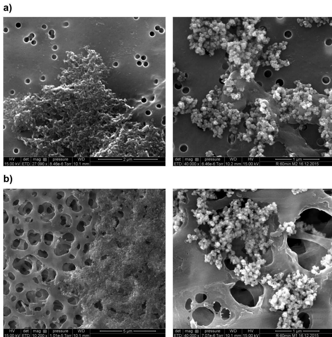
Fig. 8. SEM pictures of iron hydroxide particles retained by a) a 0.2 μm polycarbonate membrane, and b) a 0.2 μm cellulose acetate membrane. The samples were taken from the feed tank (Fig. 1a) after 1 h of aeration and filtered.
