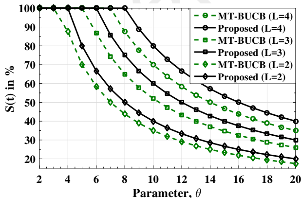
Fig. 4 Throughput of a WSN node, S(t) , in % vs. \theta .
