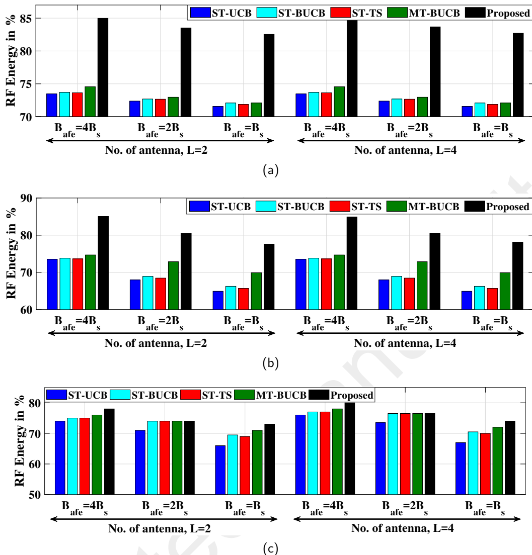
Fig. 2 Average harvested RF power in % w.r.t. genie-aided DMP for frequency band statistics (a) Case 1, (b) Case 2 and (c) Case 3.
