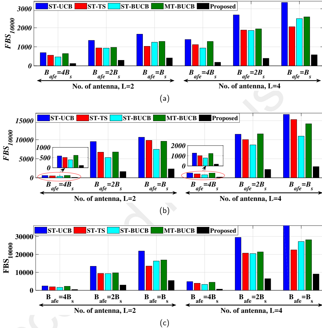
Fig. 5 Total no. of FBS for different values of L and B_s for frequency band statistics in (a) Case 1, (b) Case 2, and (c) Case 3.
