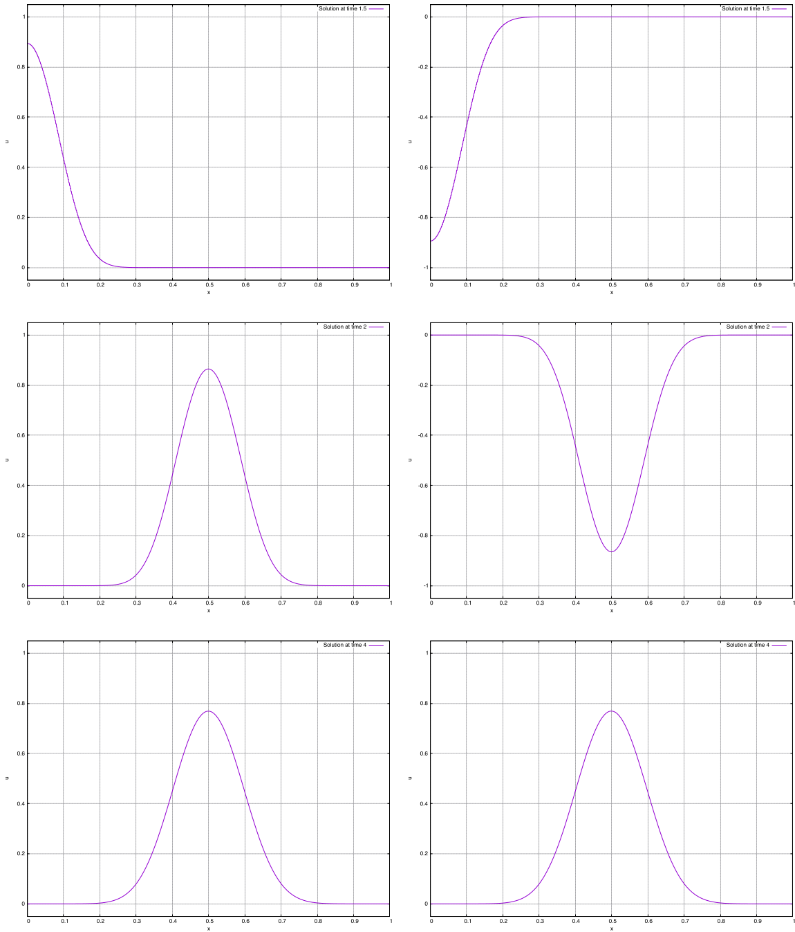
Figure 2: Numerical results: with 1000 cells on the left, 1001 cells on the right. From top to bottom: time 1.5, 2, 4.
