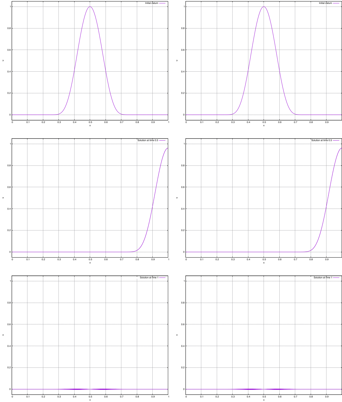
Figure 1: Numerical results: with 1000 cells on the left, 1001 cells on the right. From top to bottom: time 0, 0.5, 1.
