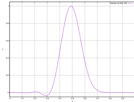
Figure 4: Solution with the Crank-Nicolson scheme ( \theta = 1/2 ) at time 100 for J = 1000
