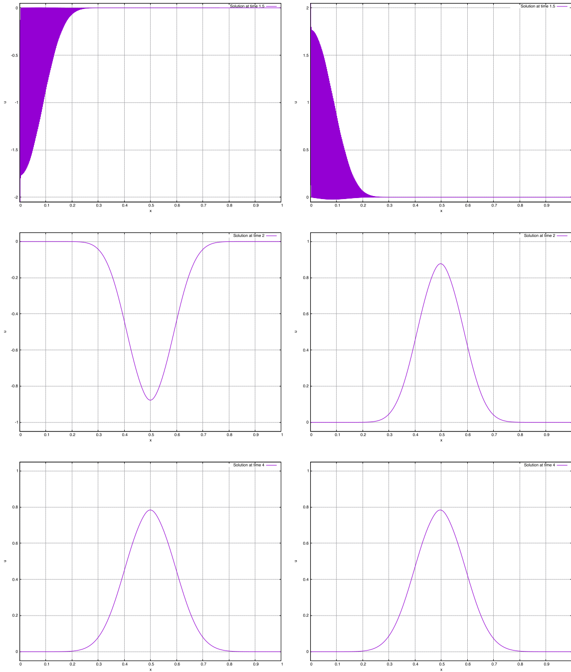
Figure 6: Numerical results: with 1000 cells on the left, 1001 cells on the right. From top to bottom: time 1.5, 2, 4.
