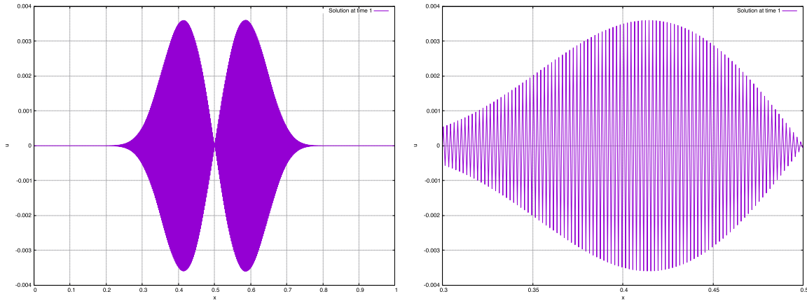
Figure 3: Zoom on the solution at time 1 for J = 1000 (see the y and x scales).
