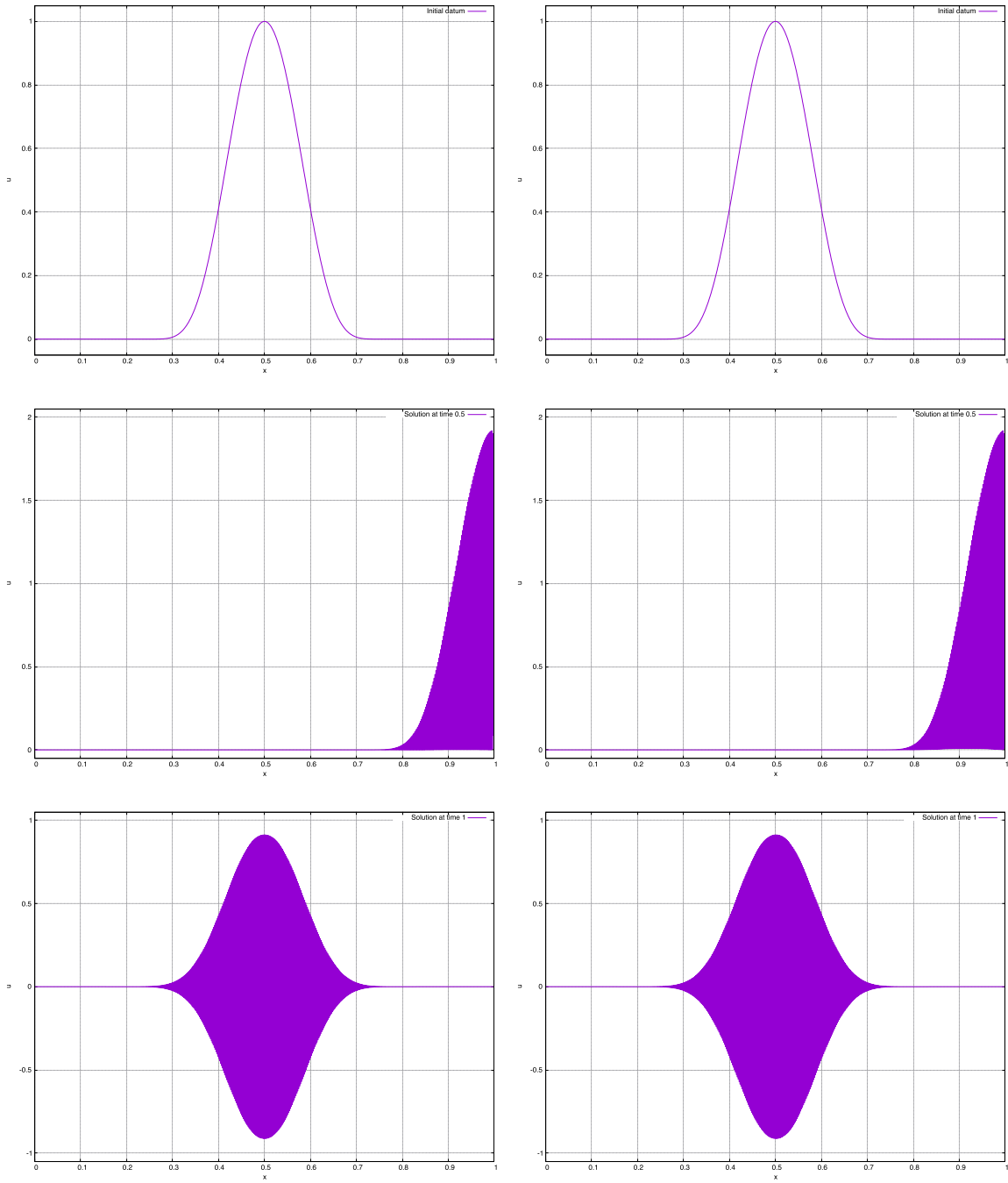
Figure 5: Numerical results: with 1000 cells on the left, 1001 cells on the right. From top to bottom: time 0, 0.5, 1.
