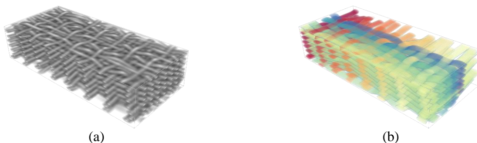
Figure 4. This procedure requires the (a) discretized representation of the virtual model and allows to compute the (b) aligned virtual model for the reference sample.
