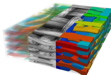
Figure 1. Different descriptors for a given 3D woven composite: CAD model (arrangement of yarns), high resolution CT image and FE mesh (yarns and resin).
