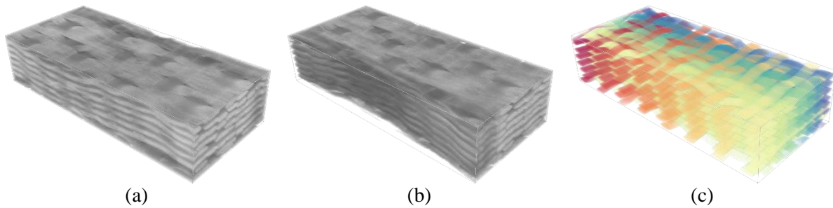
Figure 2. The results are given for the (a) reference and (b) test samples observed through CT, as well as for the (c) virtual model with the same textile definition.
