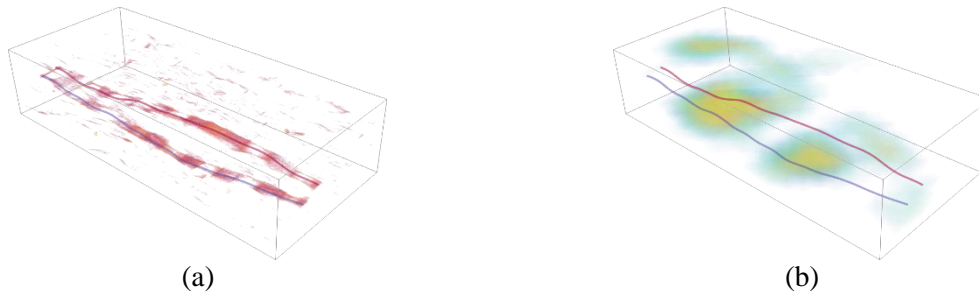
Figure 3. A good alignment is observed for the (a) semi-residual due to displacement only and (b) trace of the relative strain tensor with the intentionally missing yarns (shown as neutral fibers).
