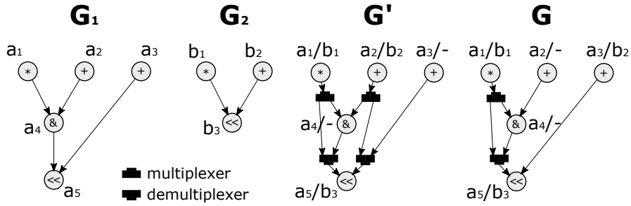
Fig. 19 The Datapath Merging Problem [60].
