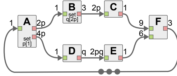
Fig. 5 Example of Schedulable Parametric Dataflow (SPDF) graph.
