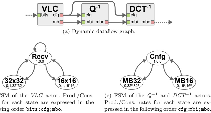
Fig. 6 Dynamic dataflow graph inspired by the residual decoding of a video decoder.
