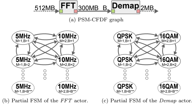
Fig. 7 PSM-CFDF graph of an OFDM demodulator used in LTE standard [16, 40, 50].
