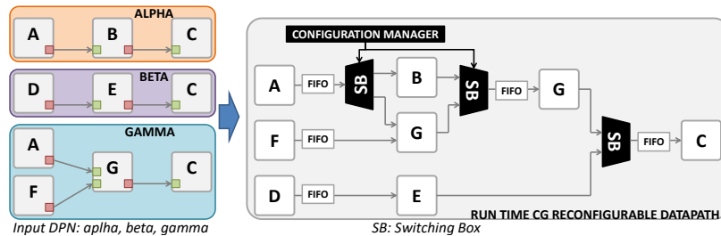
Fig. 20 Dataflow to CG reconfigurable substrate [46].
