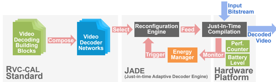
Fig. 15 Overview of an energy-aware design flow for dynamic dataflow graphs [55].
