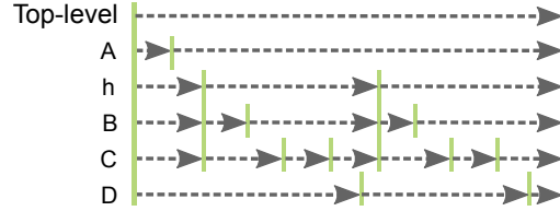
Fig. 2 Abstract representation of the quiescent points for the graph of Figure 1. Vertical lines represent quiescent points of actors. Dotpoint arrows represent actor firings and define a partial ordering of quiescent points.
