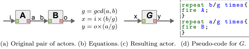
Fig. 9 Basic grouping operation used to build a quasi-static schedule.
