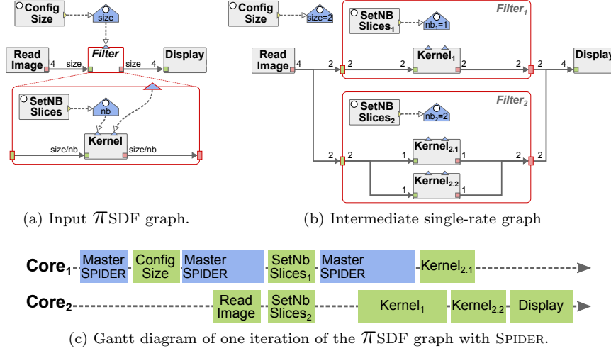
Fig. 12 Deployment process of the SPIDER runtime.
