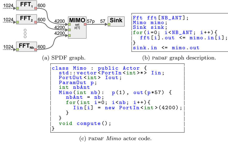
Fig. 14 Partial LTE application specification with PaDaF (From [16])
