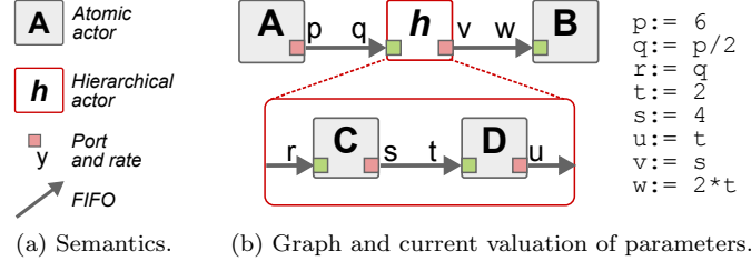
Fig. 1 Synthetic dataflow MoC implementing the reconfiguration semantics.
