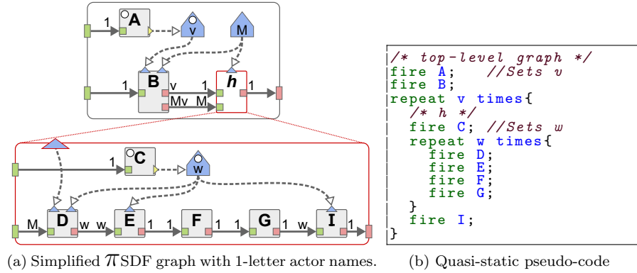
(a) Simplified \pi SDF graph with 1-letter actor names. (b) Quasi-static pseudo-code
