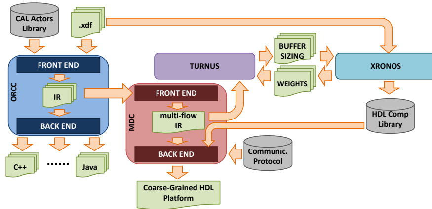
Fig. 21 Design environment for RVC-CAL compliant CG reconfigurable architectures [58].
