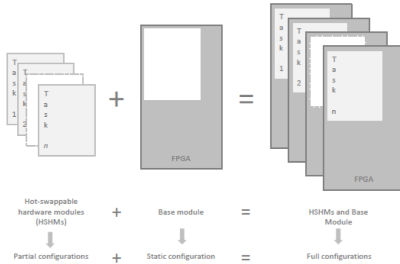
Fig. 23 Spatial and temporal partitioning of an application in a FPGA exploiting DPR [53].
