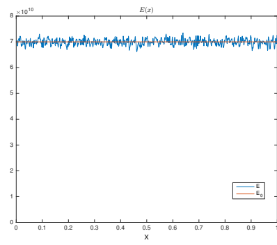
Figure 7: E(x)
