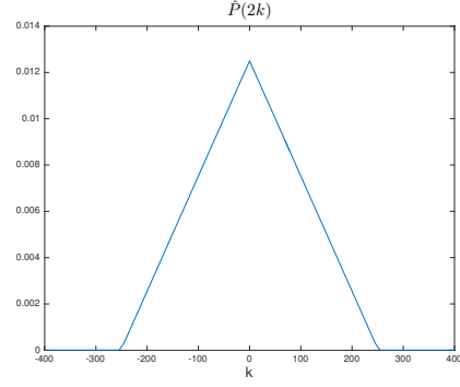
Figure 8: \hat{P}(2k)
