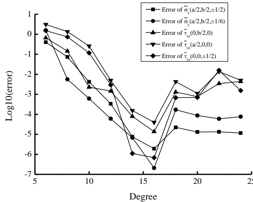
Figure 5 – The influence of the degree on the convergence. Number of collocation points = 6N .
