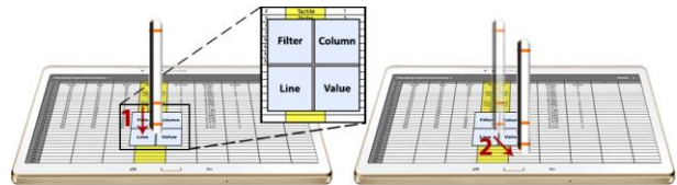
Figure 6. Technique Stack-and-Translate .
