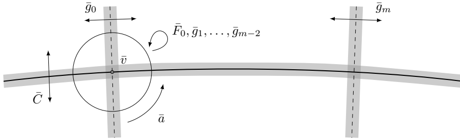
Figure 10: Lifting chains. The shaded areas represent \text{Mov}(\bar{A}, 11\bar{\delta}) , \text{Mov}(\bar{B}, 11\bar{\delta}) , and \text{Mov}(\bar{C}, 11\bar{\delta}) respectively. The isometry \bar{g}_{m-1} is not on the picture. It is not clear a priori whether it is a reflection or almost trivial at \bar{v} .
