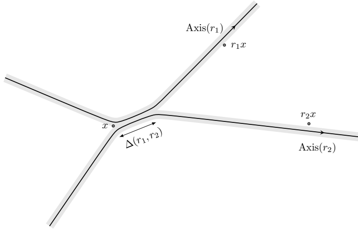
Figure 1: Overlap between two relations seen in the hyperbolic space X . The translation length \|r_i\| of r_i is roughly the distance between x and r_ix .
