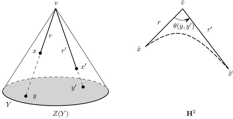
Figure 3: Geometric interpretation of the distance in the cone.
