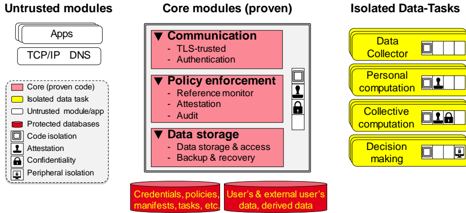
Figure 7. Logical architecture
