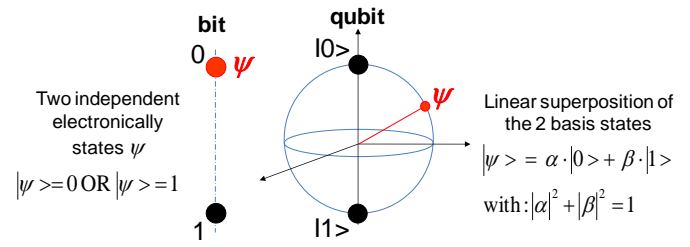
Figure 4: Values of states \psi for bit and qubit
