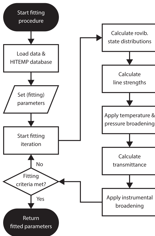
Figure 2. A calculation diagram of the developed algorithm to compute and fit non-equilibrium infrared transmittance spectra. The left hand column represents the preparation of the calculation, including the users choice (parallelogram) of to be fitted parameters. The fitting iteration process that involves the calculation of the spectra, is elaborated in the right hand column. The fit is completed when one of the function, step, or optimality tolerances is satisfied, all with a relative value of 10^{-6} .
