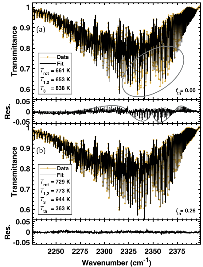
Figure 4. Two fits on the same CO 2 and CO data at 2 ms in the discharge with a 5–10 ms on–off duty cycle at 50 mA and 6.7 mbar. In panel (a) f_{\text{th}} = 0 , assuming a non-thermal population over the whole reactor, while in (b) f_{\text{th}} = 0.26 . The residual is shown on the same scale as the data.
