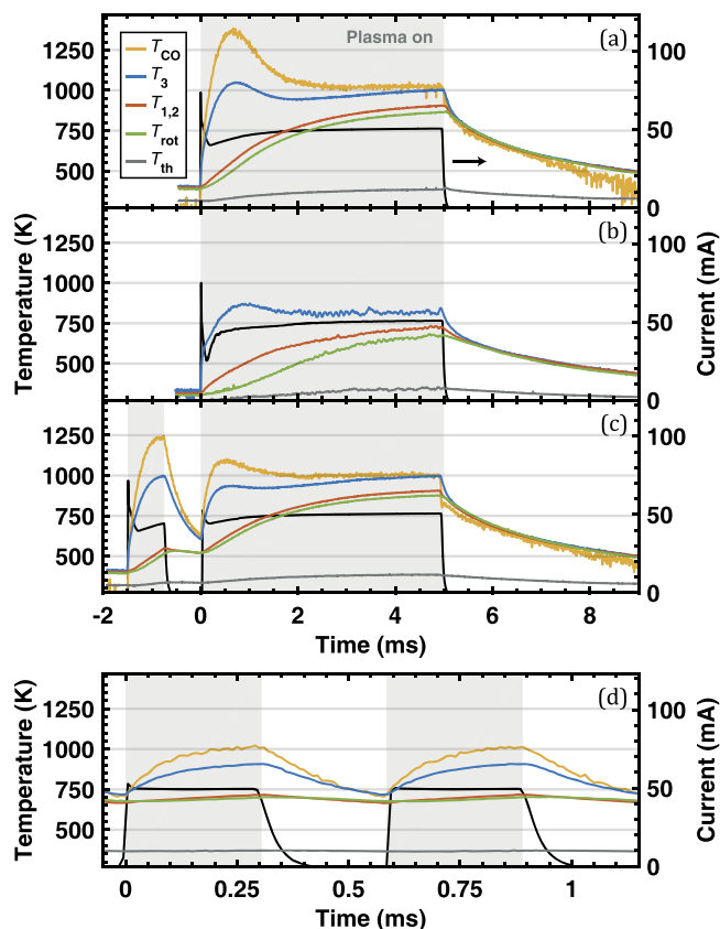
Figure 7. Four time-resolved measurement series at a pressure of 6.7 mbar and plasma current of 50 mA. The plasma current and fitted temperatures are plotted versus time. (a) 5–10 ms on-off measurement, same as in figure 5. (b) Single-pulse measurement, in which the off-time is increased to 150 ms to remove most of the CO and O 2 before the next discharge. (c) 0.75–0.75–5–10 ms on-off-off measurement. The same as (a), but with a 0.75–0.75 ms on-off pre-pulse. (d) 0.3–0.3 ms on-off (two periods are shown).
