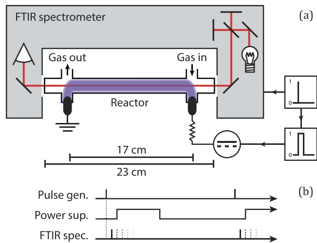
Figure 1. (a) The FTIR spectrometer, including the plasma reactor, positioned in the sample compartment. A pulse generator is used to simultaneously trigger the step-scan mode of the spectrometer and the square DC pulse for the plasma. The trigger scheme is shown in (b).
