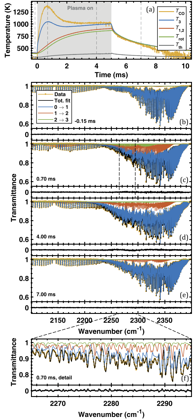
Figure 5. A time-resolved measurement series at a pressure of 6.7 mbar, plasma current of 50 mA, and a 5–10 ms on–off sequence. Panel (a) shows the fitted temperatures versus time. The dashed lines indicate the time points for which the fit on the data is displayed in panels (b)–(e). Residuals are shown below each panel. \text{CO}_2 and \text{CO} lines are mostly located at energies respectively larger and smaller than 2235 \text{ cm}^{-1} . Contributions to the fit corresponding to transitions of \nu_3 or \nu_{\text{CO}} of 0 \rightarrow 1 , 1 \rightarrow 2 , and 2 \rightarrow 3 are shown separately. Panel (f) shows a detail of panel (c).
