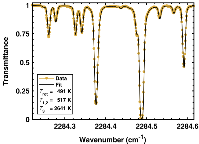
Figure 3. A fit, using the algorithm, on CO 2 data from Dang et al [9]. Transmission data is digitally extracted from the article and divided by an artificial background.
