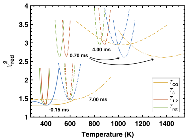
Figure 6. The reduced chi-squared for varying T_{rot} , T_{1,2} , T_3 , and T_{CO} individually. The same time points are used as in figure 5. Time points are grouped in line style, while color indicates the tested temperature.
