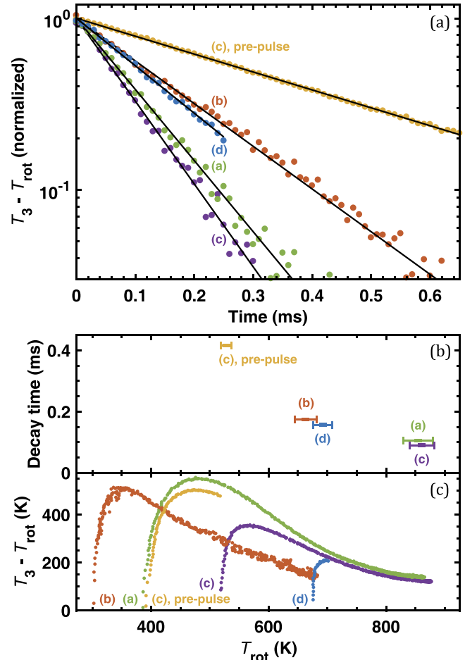
Figure 8. (a) Normalized relaxation of T_3 to T_{\text{rot}} versus time after plasma off. The labels correspond to the panel labels of figure 7. The black solid lines represent the fitted exponential decay. (b) The characteristic decay times versus the rotational temperature during relaxation. (c) The elevation of T_3 with respect to T_{\text{rot}} versus the rotational temperature, during the plasma-on phases of figure 7.
