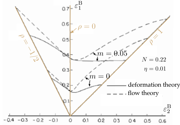
Figure 9: Examples of forming limit diagrams predicted for the two multiaxial constitutive models (5.2) and (5.3) taken from Hutchinson and Neale (1978b). The curves are based on the long-wavelength approximation for the maximum strains attained outside the neck under biaxial stretching imposed on the sheet outside the neck with \varepsilon_2^B = \rho \varepsilon_1^B .
