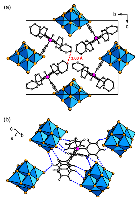
Figure 1. (a) Mixed polyhedral and ball-and-stick representations of the crystal packing in (1)_2[W_6O_{19}] (H-atoms are omitted for clarity). The red dotted line corresponds to the shortest intermolecular C...C distance. (b) Representation of the fourteen strong C-H...O contacts (blue dotted lines) in (1)_2[W_6O_{19}] . (blue octahedra = WO_6 , grey sphere: carbon, pink sphere: phosphor, gold sphere: oxygen, white sphere: hydrogen).
