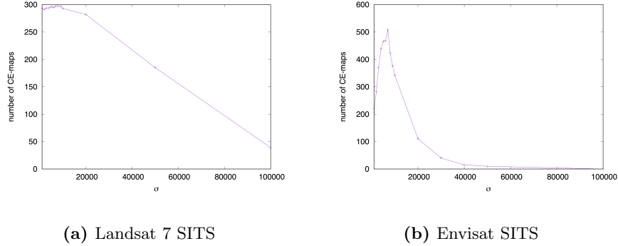
Fig. 4 Number of CE-maps vs. minimum support threshold \sigma
