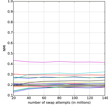
(a) NMI variation of the top-20 highest rank CE-maps
