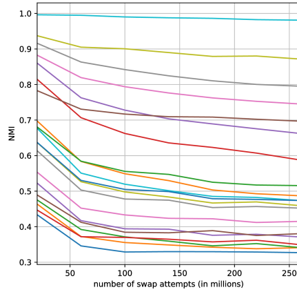
(a) NMI variation of the top-20 highest rank CE-maps, |\mathcal{D}| = 6
