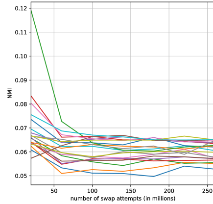
(b) NMI variation of the top-20 lowest rank CE-maps, |\mathcal{D}| = 6
