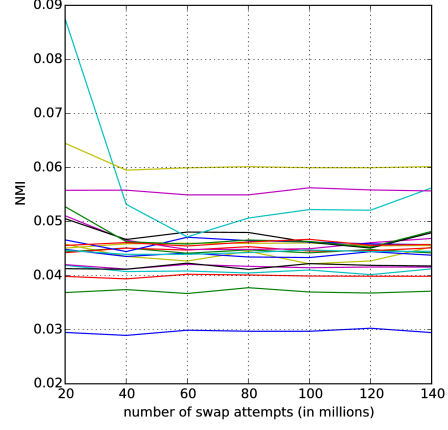
(b) NMI variation of the top-20 lowest rank CE-maps
