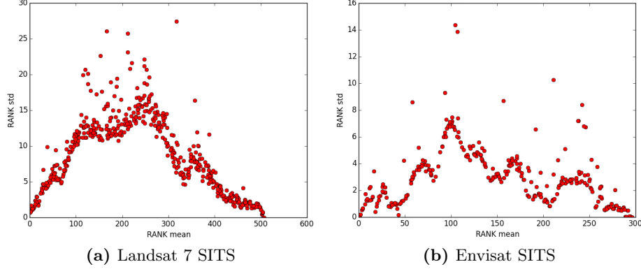
Fig. 9 Ranking stability: rank std. vs. rank mean
