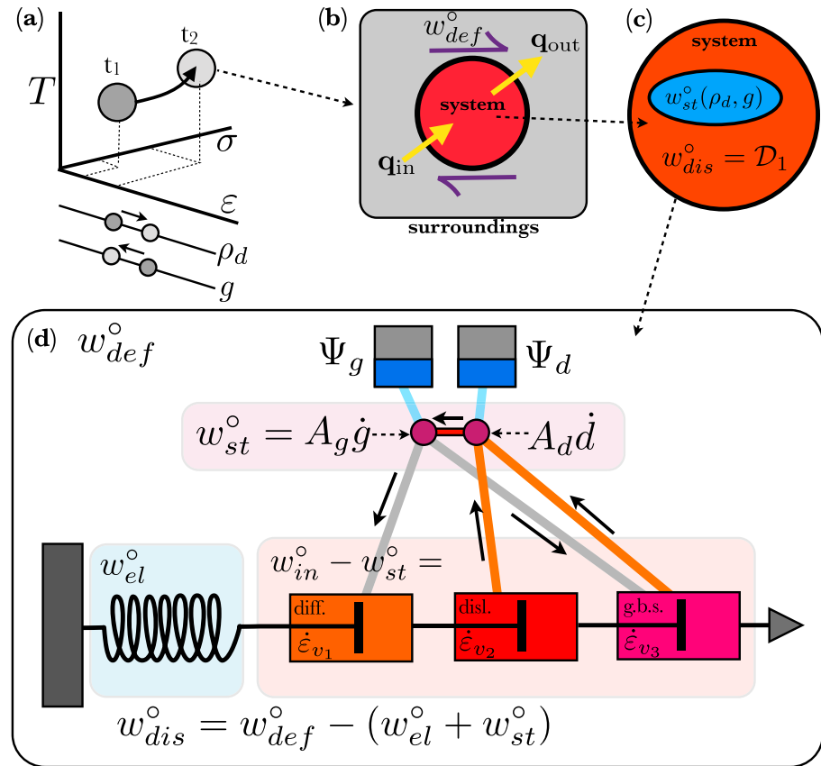
Figure 5. Schematic of the model, with work rates defined in Table 2. (a) Two states in T - \varepsilon - \sigma - \rho_d - g space, connected by a path with irreversible dissipation. The \varepsilon is the total strain, but \varepsilon_v (not shown) is also needed to describe the state. (b) In the 0-D thermodynamic system of interest here, deformation (work) is applied to a representative elementary volume (orange circle), which is open to heat but not mass. (c) Inside the representative elementary volume, energy can be stored or dissipated. (d) The mechanical model consists of a Maxwell body with three nonlinear creep mechanisms and two microstructural state variables, dislocation density, and grain size. Lines indicate couplings; grey: diffusion creep and grain boundary sliding depend nonlinearly on grain size; orange: dislocation and grain boundary sliding creep both involve dislocation production and motion. Some of those dislocations go into changing the grain size (red line). Any changes in mean dislocation density and grain size involve dissipated energy (purple dots) and a change in the stored energy (blue tanks).
