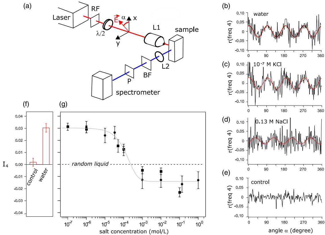
FIG. 1. Polarized second harmonic scattering experiments. (a) Experimental setup. A femtosecond laser beam is focused into a water cuvette through a red filter (RF), a half-wave plate, and a microscope objective (L1). The harmonic photon is detected at a right angle through a lens (L2), a blue filter (BF), and a vertical polarizer (P). The black line represents the residue of the signal at the frequency 4\alpha , the red line corresponds to the fit for (b) neat water, (c) 10^{-7} M KCl, (d) 0.13 M NaCl, and (e) diluted molecule DiA in ethanol, where no correlations are expected. (f) Magnitude of I_4 for molecule DiA and water. (g) I_4 for different KCl (square) and NaCl (round) concentrations. I_4 is positive when the frequency 4\alpha residue is positive at \alpha = 0 and negative when the frequency 4\alpha residue is negative at \alpha = 0 . The dashed line indicates I_4 = 0 corresponding to a pure random fluid. The gray line helps the reader. \alpha = 0 indicates that the laser beam is vertically polarized.
